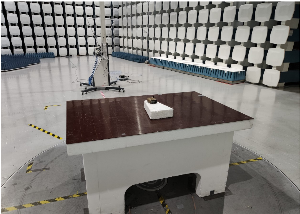
Radiated Emissions, 30 - 1000 MHz
