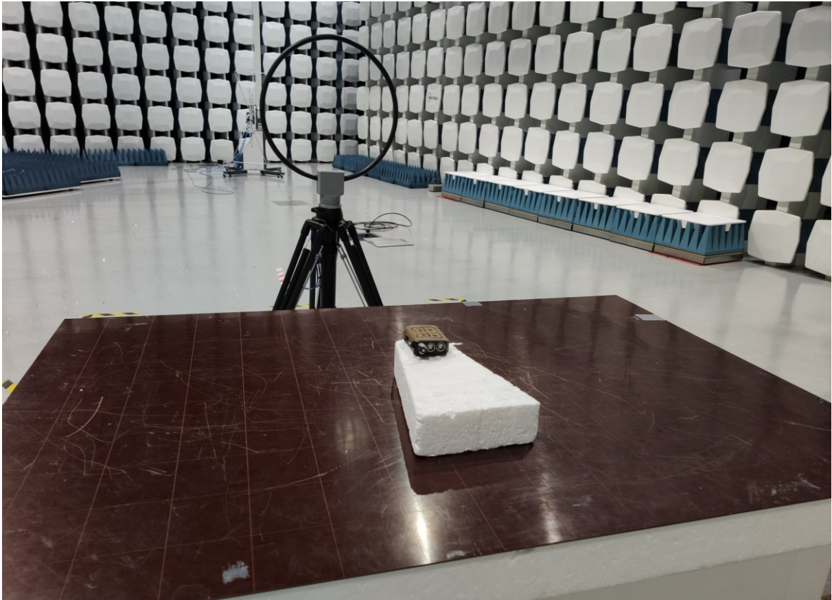
Radiated Emissions, Below 30 MHz
