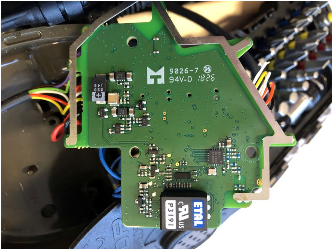
backside of the left PCB
