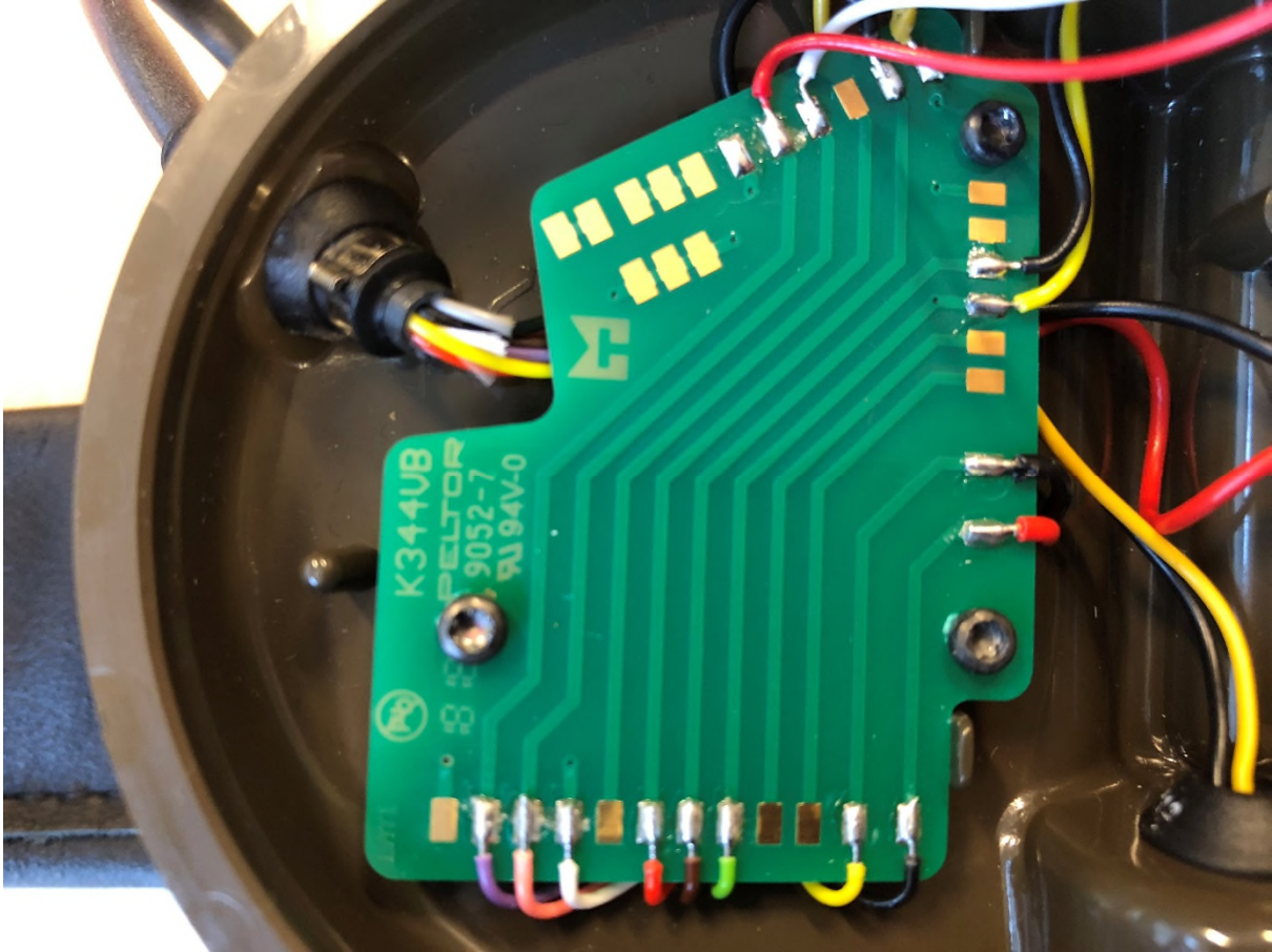
frontside of the right PCB
