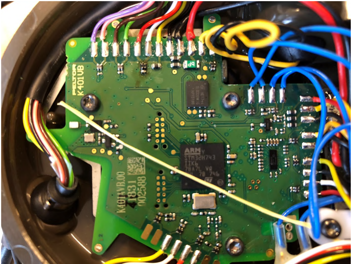
frontside of the left PCB
