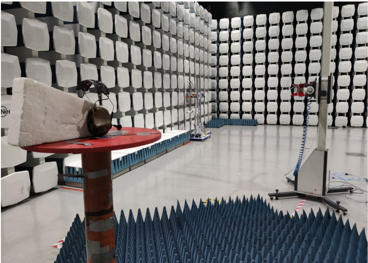
Radiated Emissions, 1 - 10 GHz
