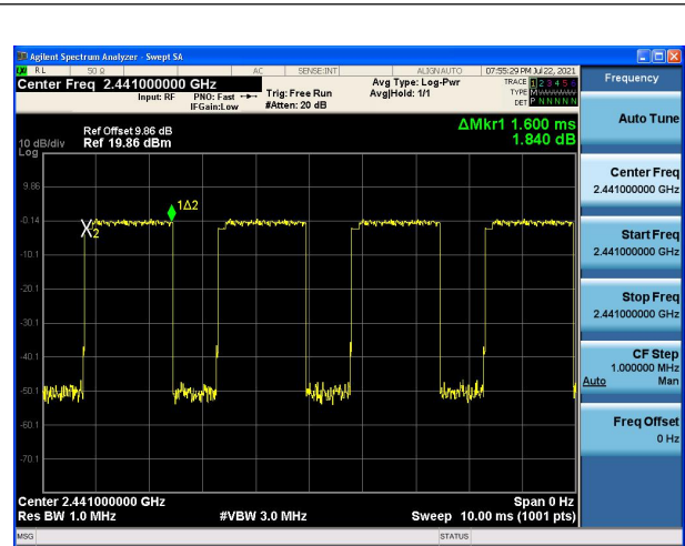
Modulation: 8DPSK 3DH3 2441
