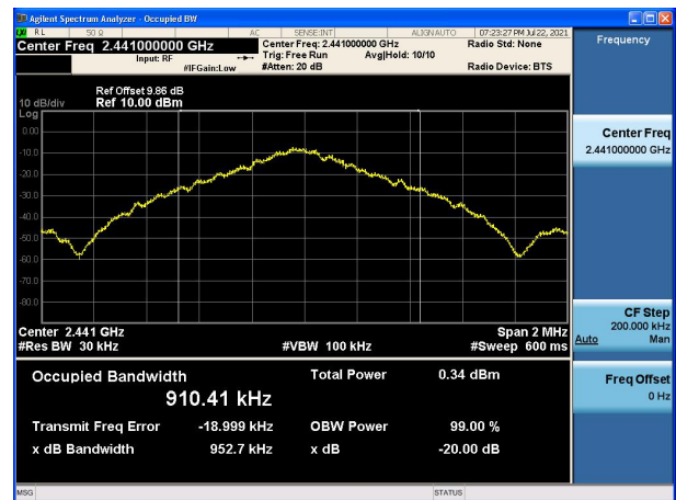
Modulation: GFSK 2441MHz
