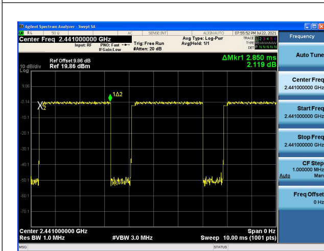
Modulation: 8DPSK 3DH5 2441
