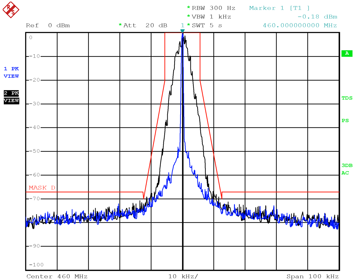
Emission mask D with modulation DMR 4FSK at 460 MHz
