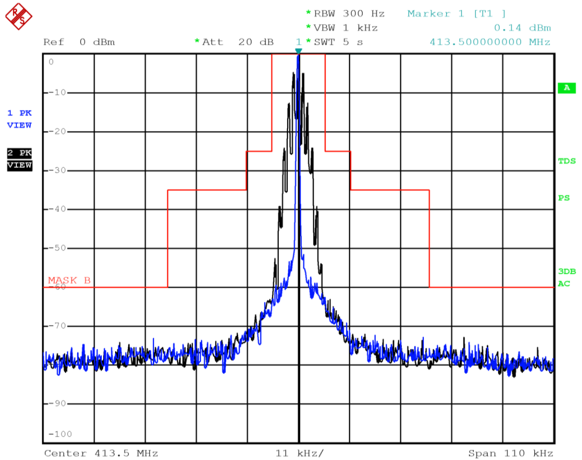
Emission mask B with modulation FM 12.5 kHz at 413.5 MHz
