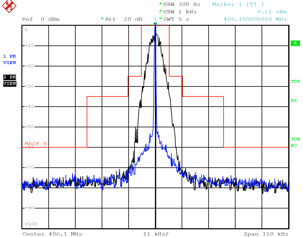
Emission mask B with modulation DMR 4FSK at 406.1 MHz
