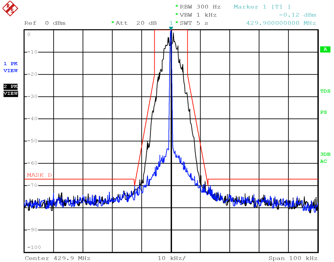
Emission mask D with modulation DMR 4FSK at 429.9 MHz
