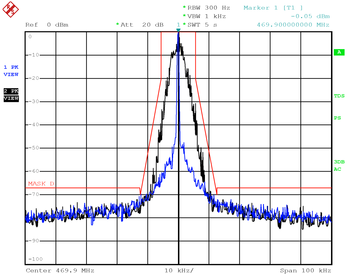
Emission mask D with modulation DMR 4FSK at 469.9 MHz
