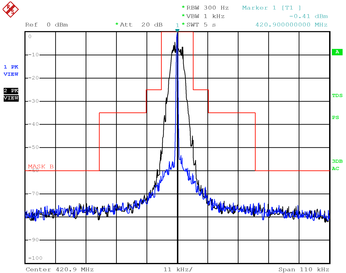
Emission mask B with modulation P25 C4FM at 420.9 MHz
