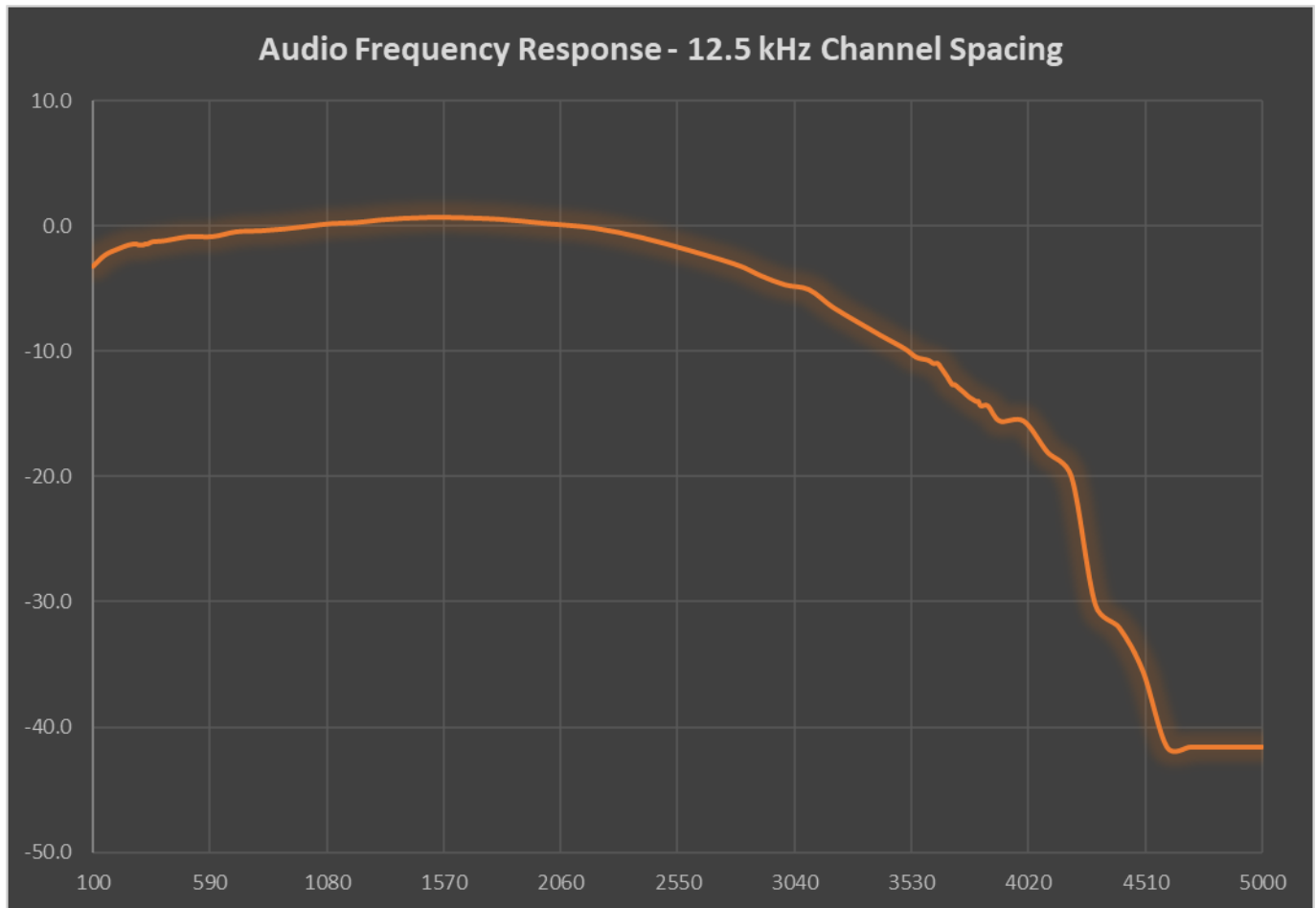
Audio frequency response at 413.5 MHz (12.5 kHz)
