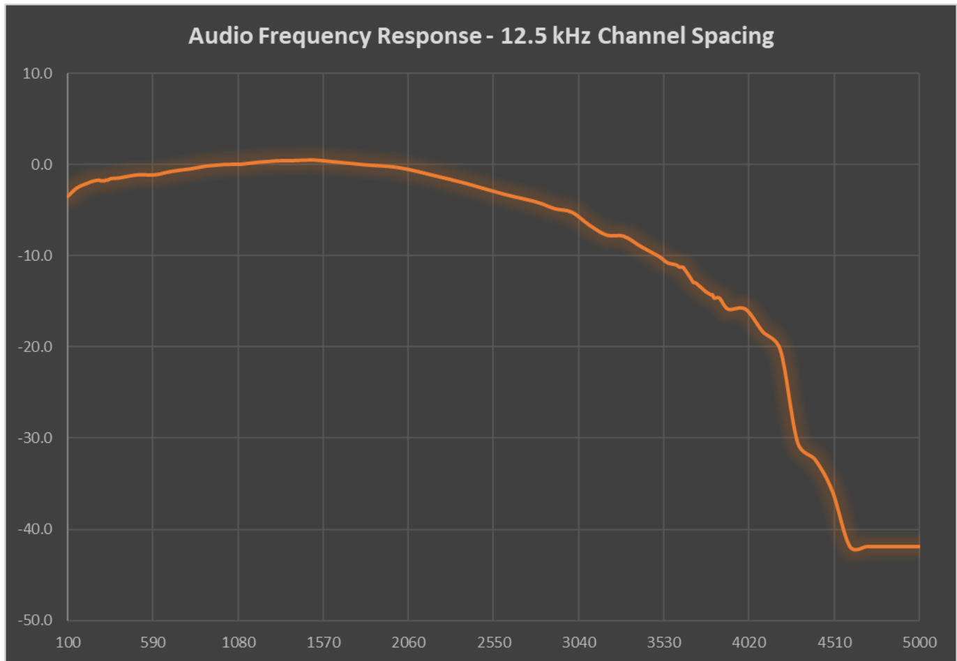
Audio frequency response at 460.0 MHz (12.5 kHz)
