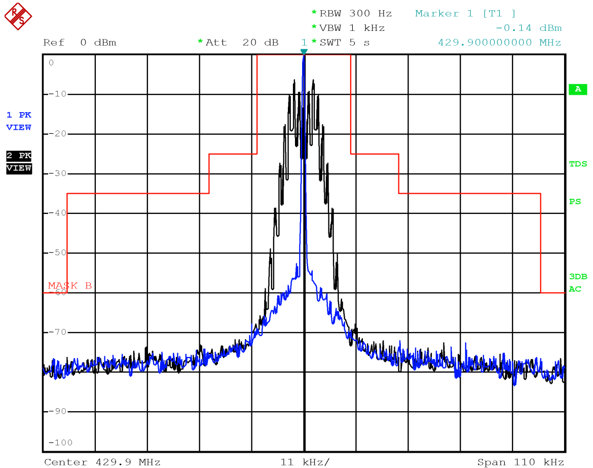
Emission mask B with modulation FM 25 kHz at 429.9 MHz
