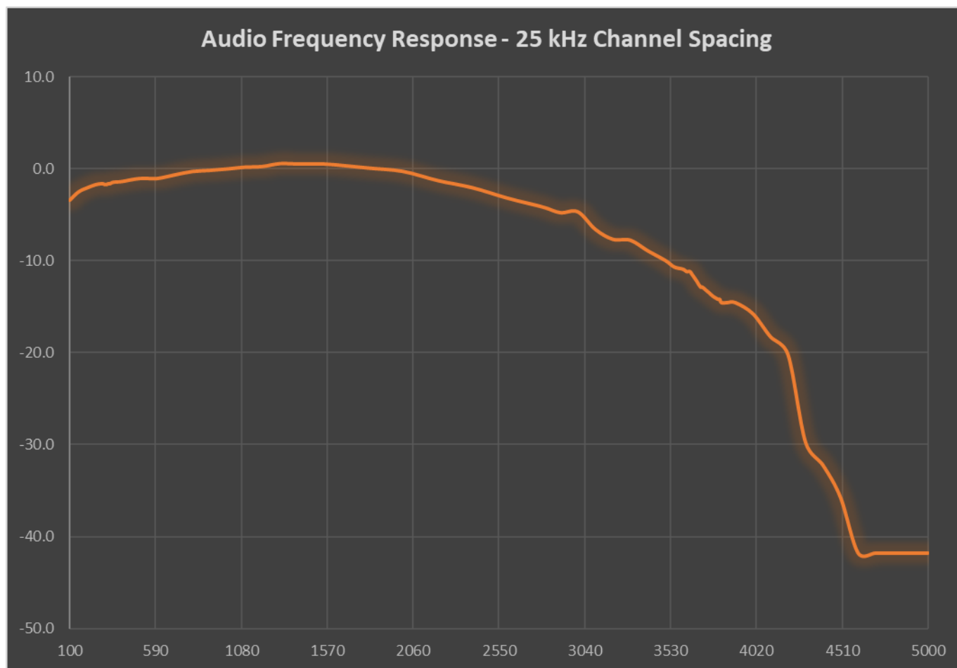
Audio frequency response at 460.0 MHz (25 kHz)
