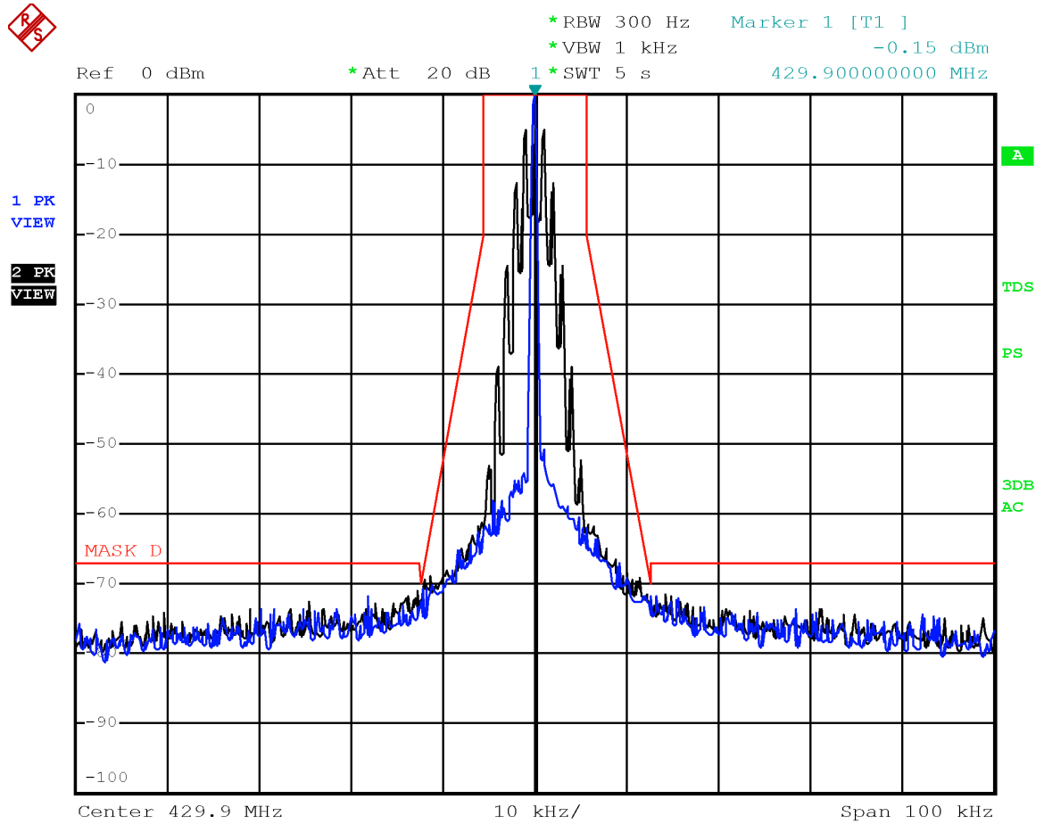
Emission mask D with modulation FM 12.5 kHz at 429.9 MHz
