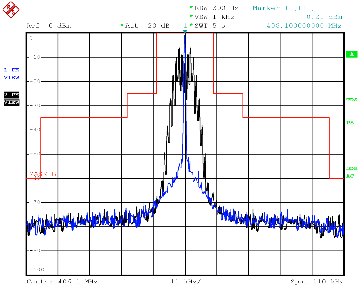
Emission mask B with modulation FM 25.0 kHz at 406.1 MHz
