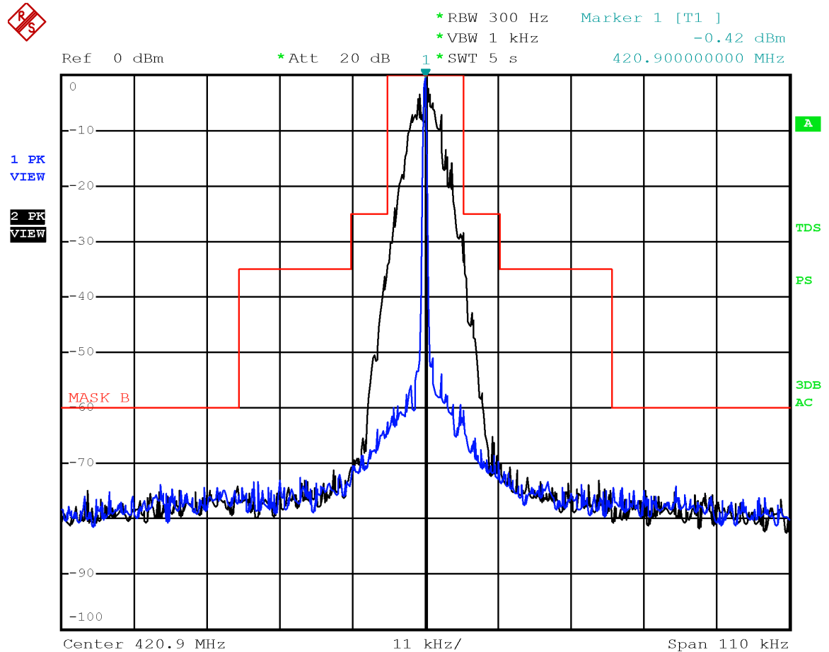
Emission mask B with modulation DMR 4FSK at 420.9 MHz
