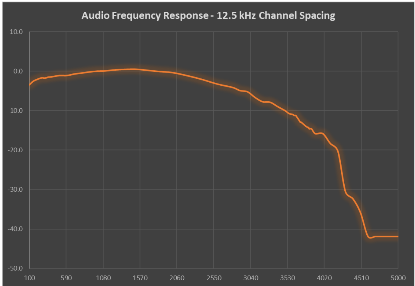
Audio frequency response at 421.1 MHz (12.5 kHz)
