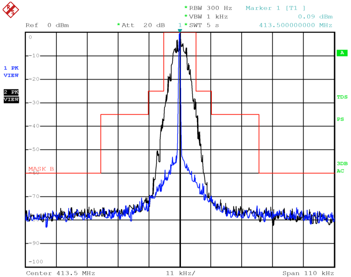
Emission mask B with modulation DMR 4FSK at 413.5 MHz
