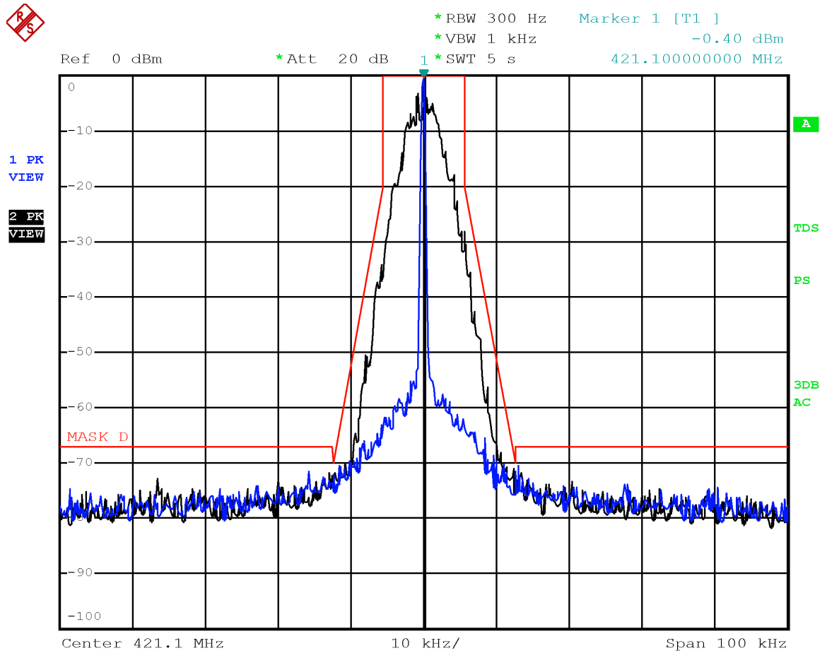
Emission mask D with modulation DMR 4FSK at 421.1 MHz
