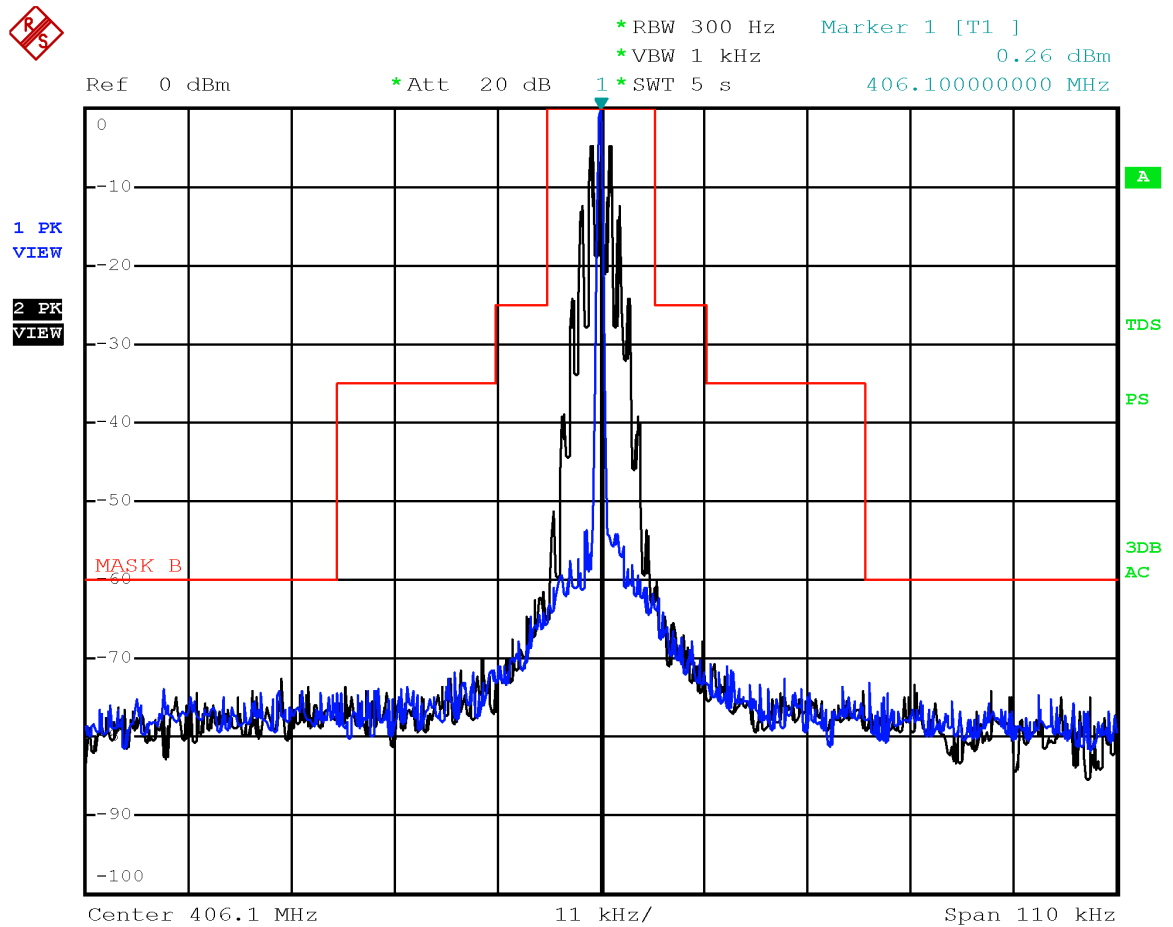
Emission mask B with modulation FM 12.5 kHz at 406.1 MHz
