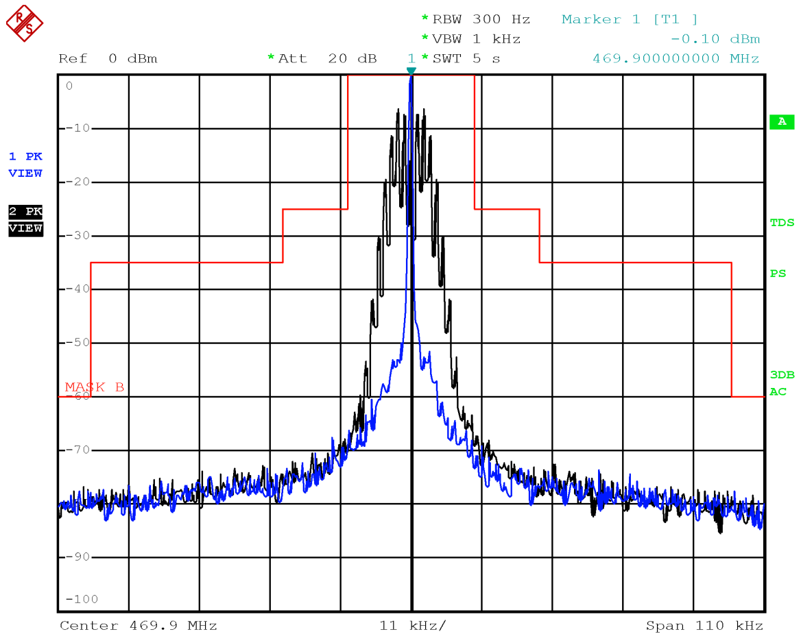
Emission mask B with modulation FM 25 kHz at 469.9 MHz
