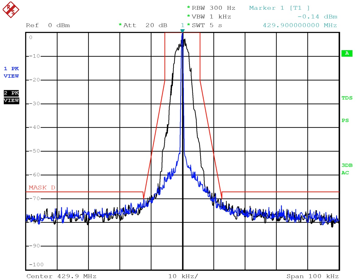
Emission mask D with modulation P25 C4FM at 429.9 MHz
