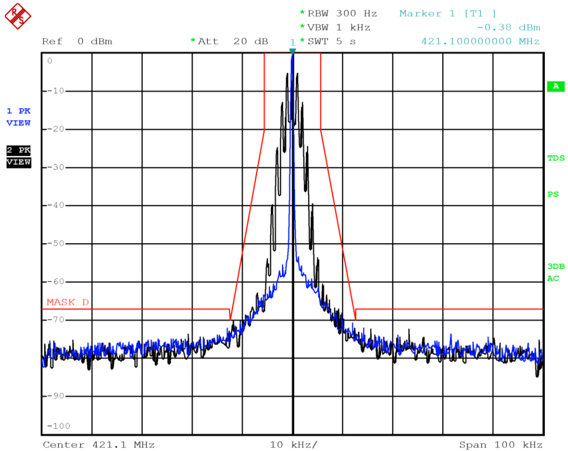
Emission mask D with modulation FM 12.5 kHz at 421.1 MHz
