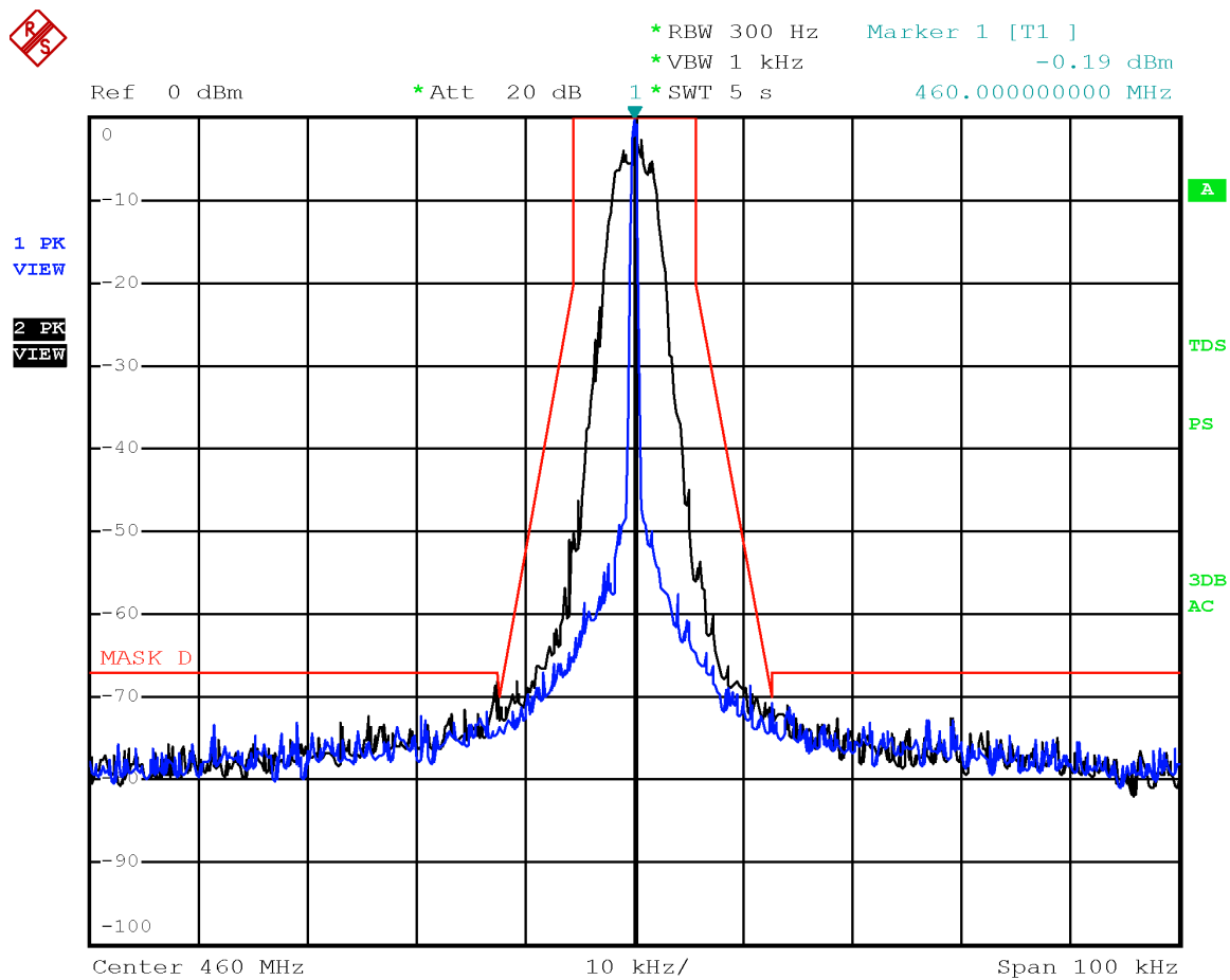
Emission mask D with modulation P25 C4FM at 460 MHz
