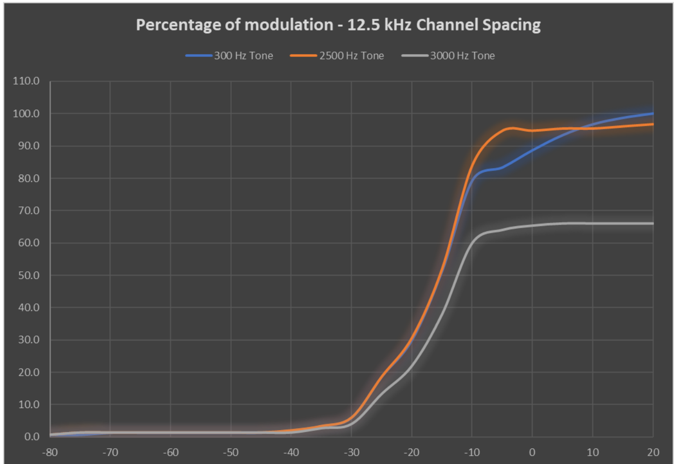
Modulation Limiting at 413.5 MHz (12.5 kHz)
