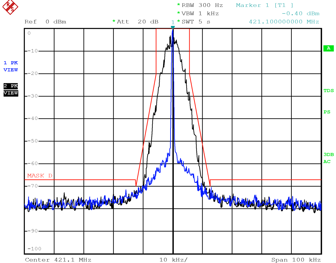
Emission mask D with modulation P25 C4FM at 421.1 MHz
