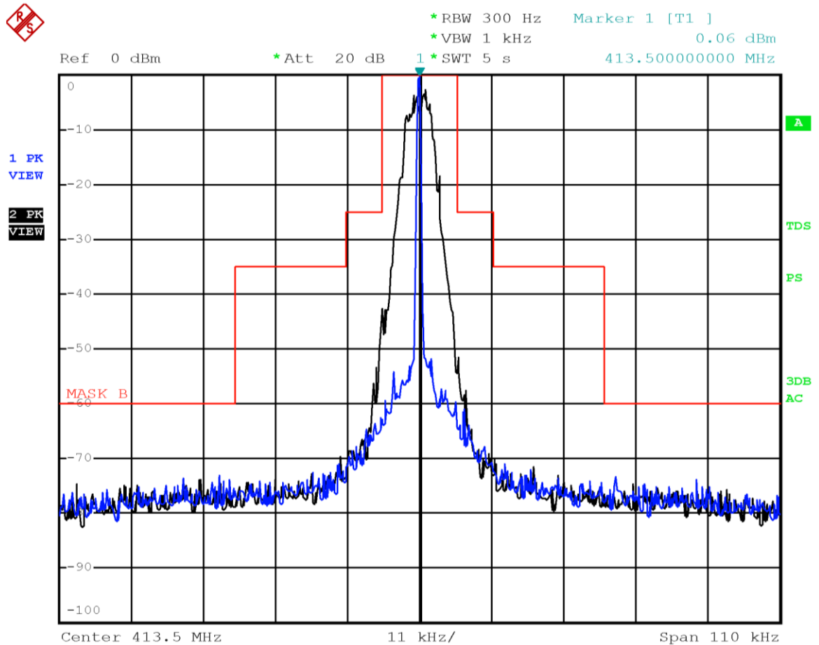
Emission mask B with modulation P25 C4FM at 413.5 MHz
