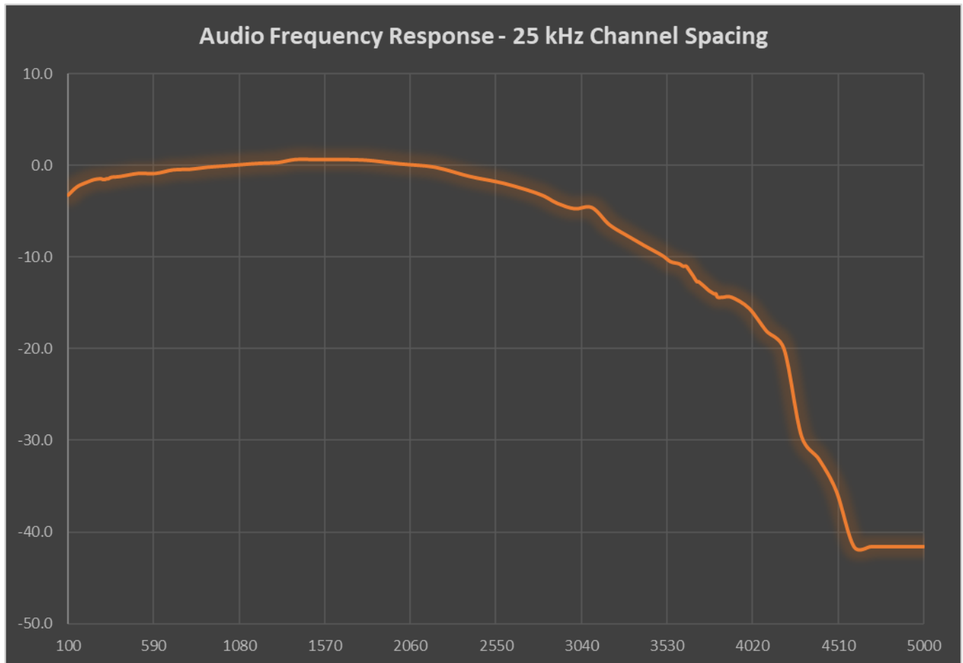
Audio frequency response at 413.5 MHz (25 kHz)
