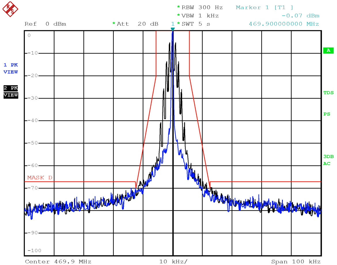
Emission mask D with modulation FM 12.5 kHz at 469.9 MHz
