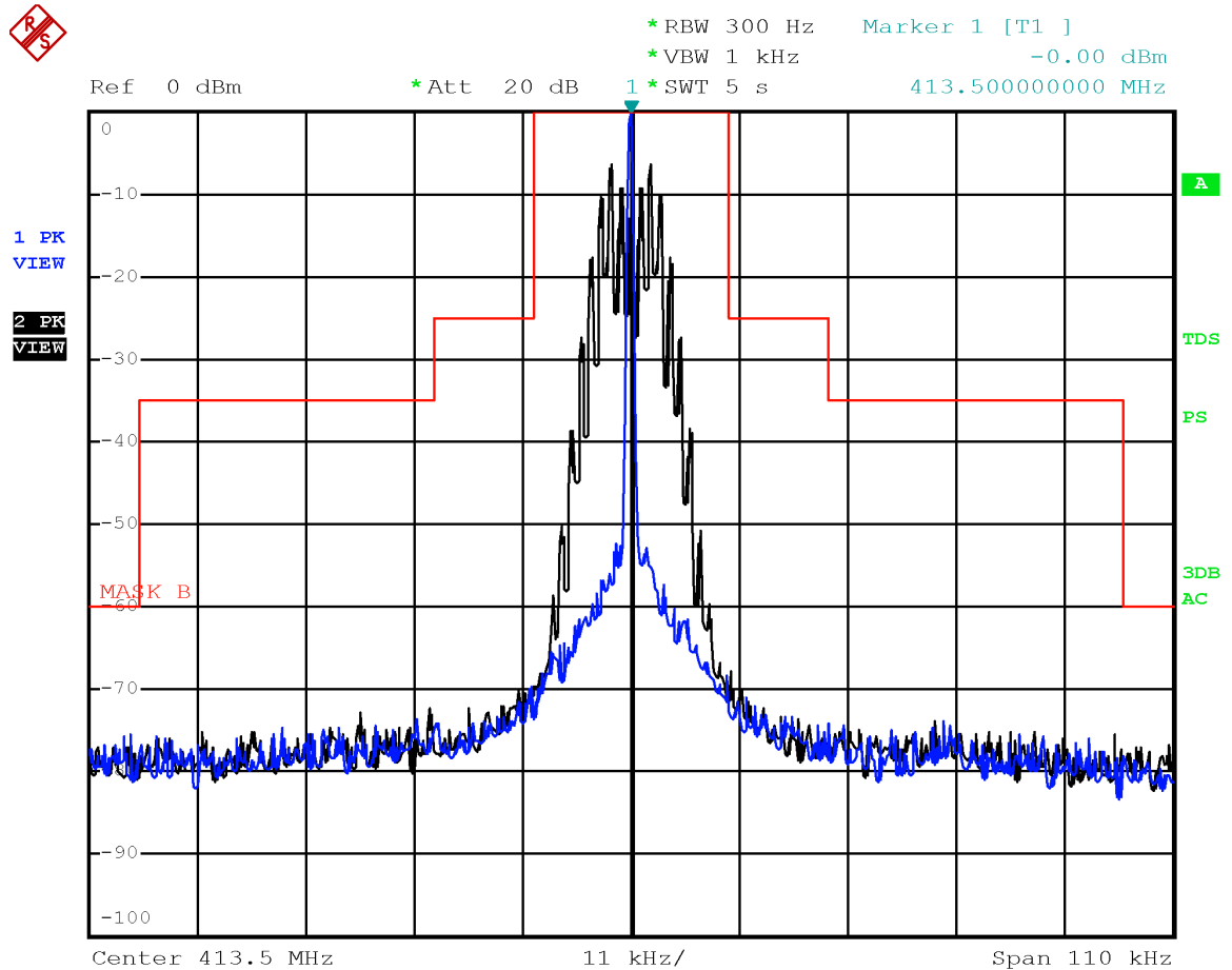
Emission mask B with modulation FM 25 kHz at 413.5 MHz
