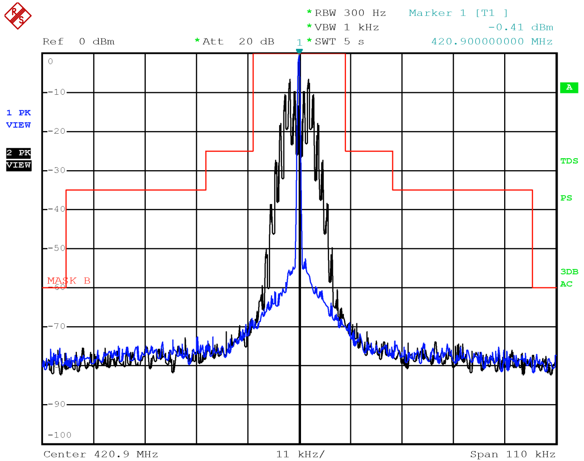
Emission mask B with modulation FM 25 kHz at 420.9 MHz
