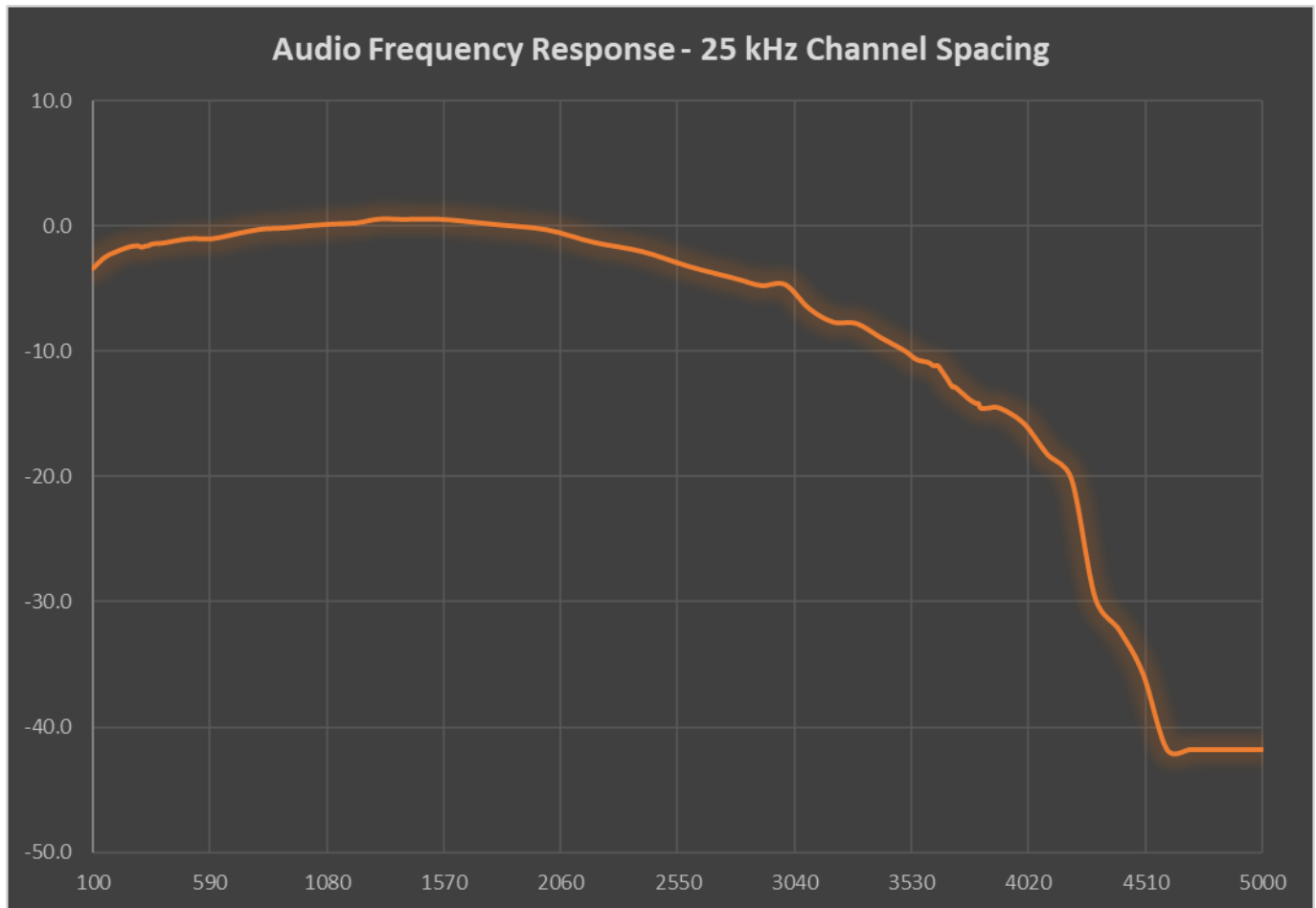
Audio frequency response at 421.1 MHz (25 kHz)
