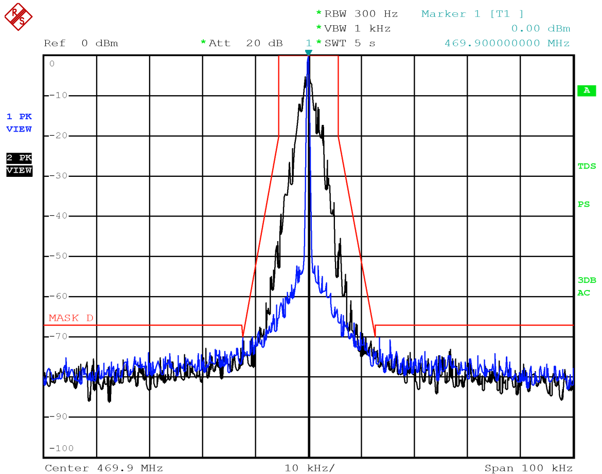
Emission mask D with modulation P25 C4FM at 469.9 MHz
