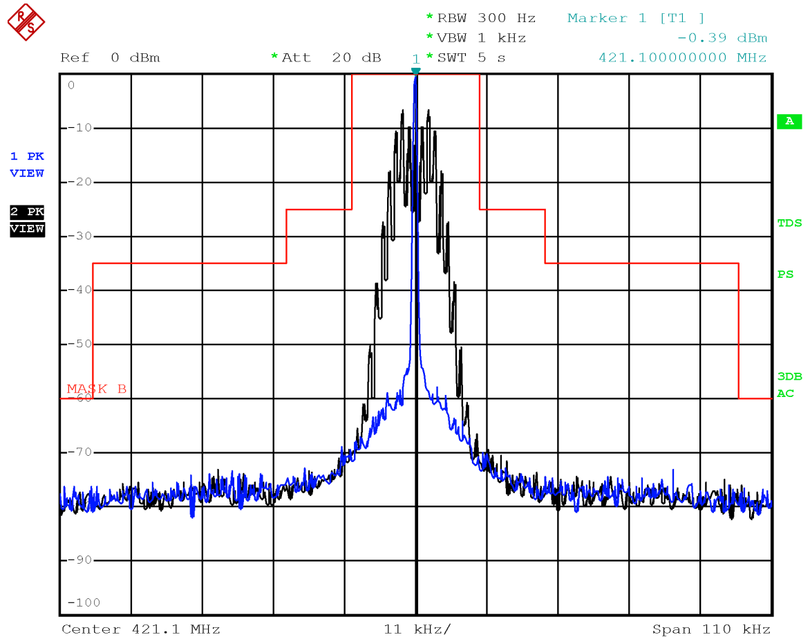
Emission mask B with modulation FM 25 kHz at 421.1 MHz
