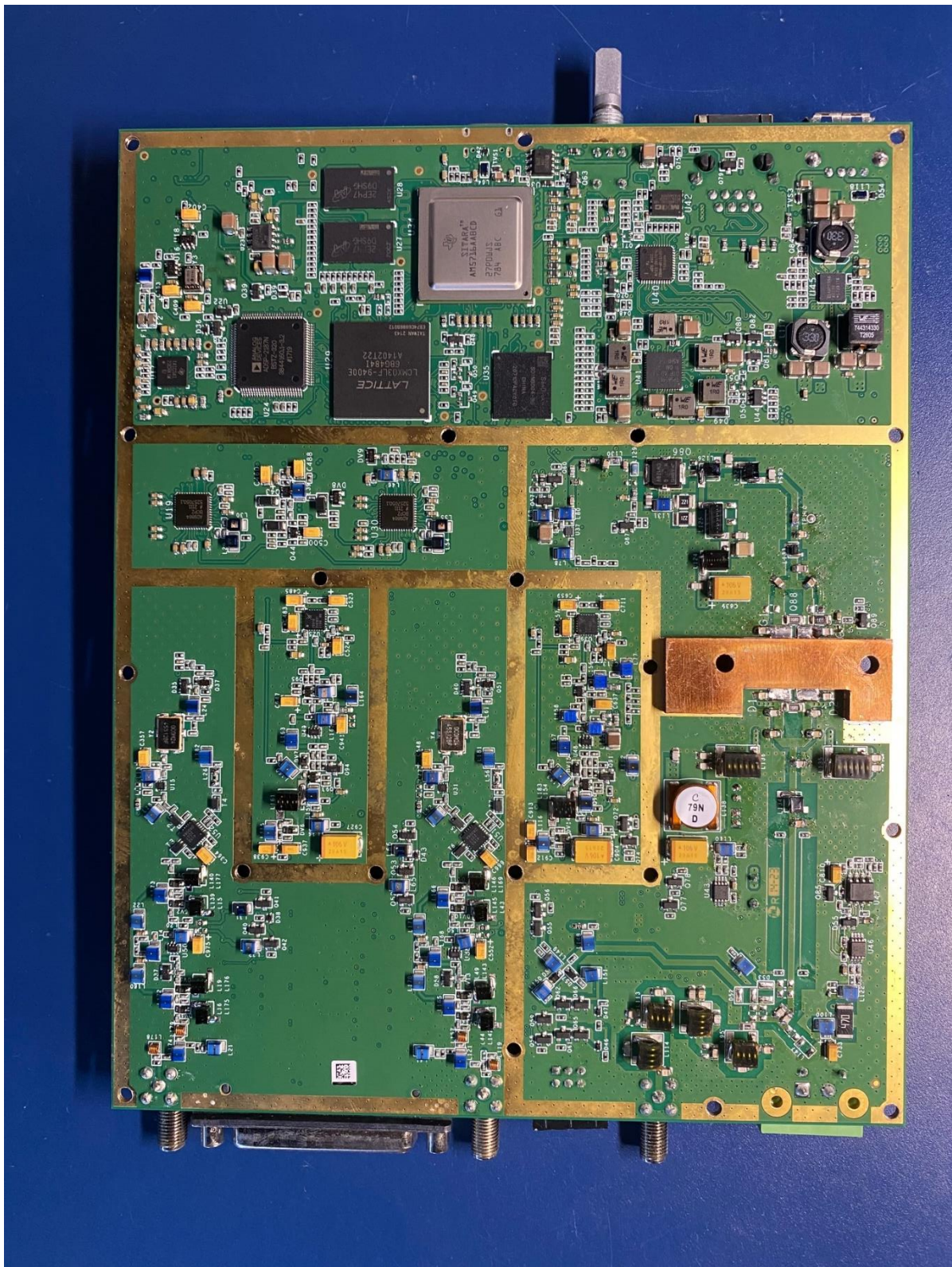
KA-450e Main board (bottom view)
