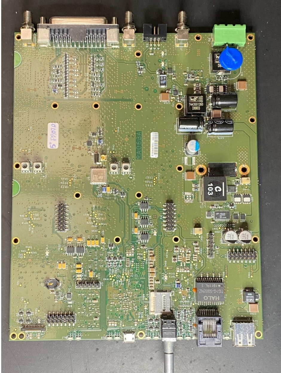
KA-160e Main board (top view)
