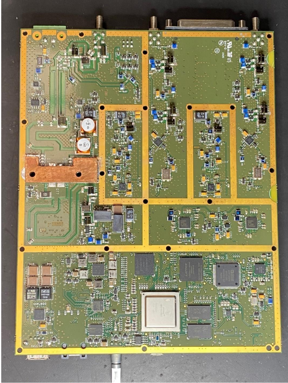
KA-160e Main board (bottom view)
