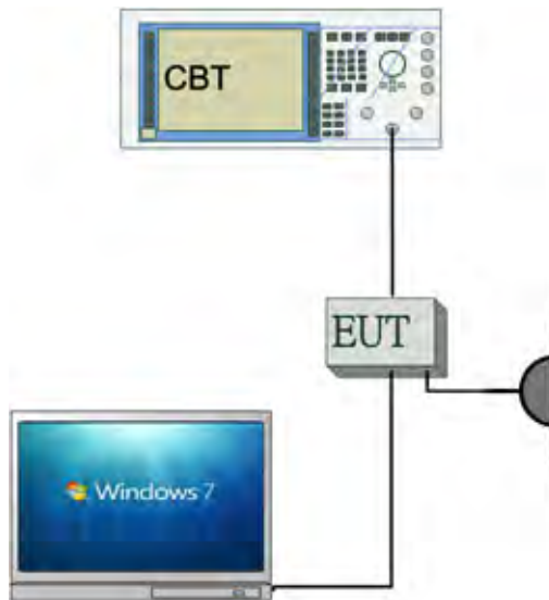
Fig. 2-2 Conducted (Antenna Port) Configuration
