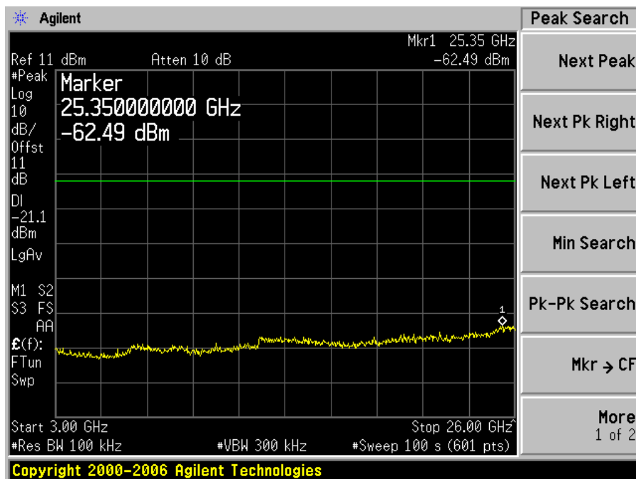
Plot 2: 3 ~26 GHz
