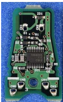
Front (PCB)
