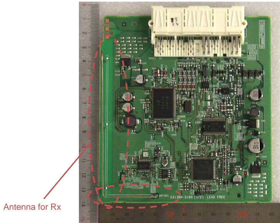
Component side
