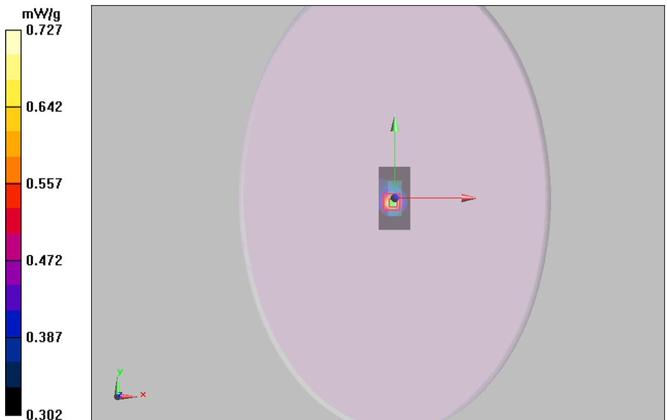
Figure 13 802.11n(HT20) with IBM T61 Test Position 1 Channel 11
