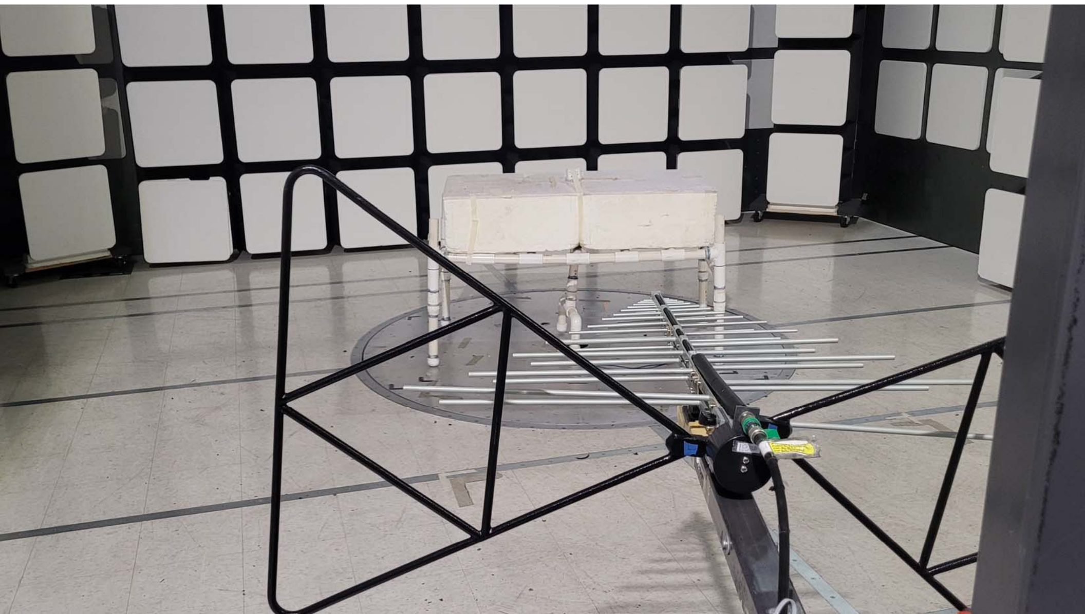
Radiated Emissions - Below 1 GHz - Front View
