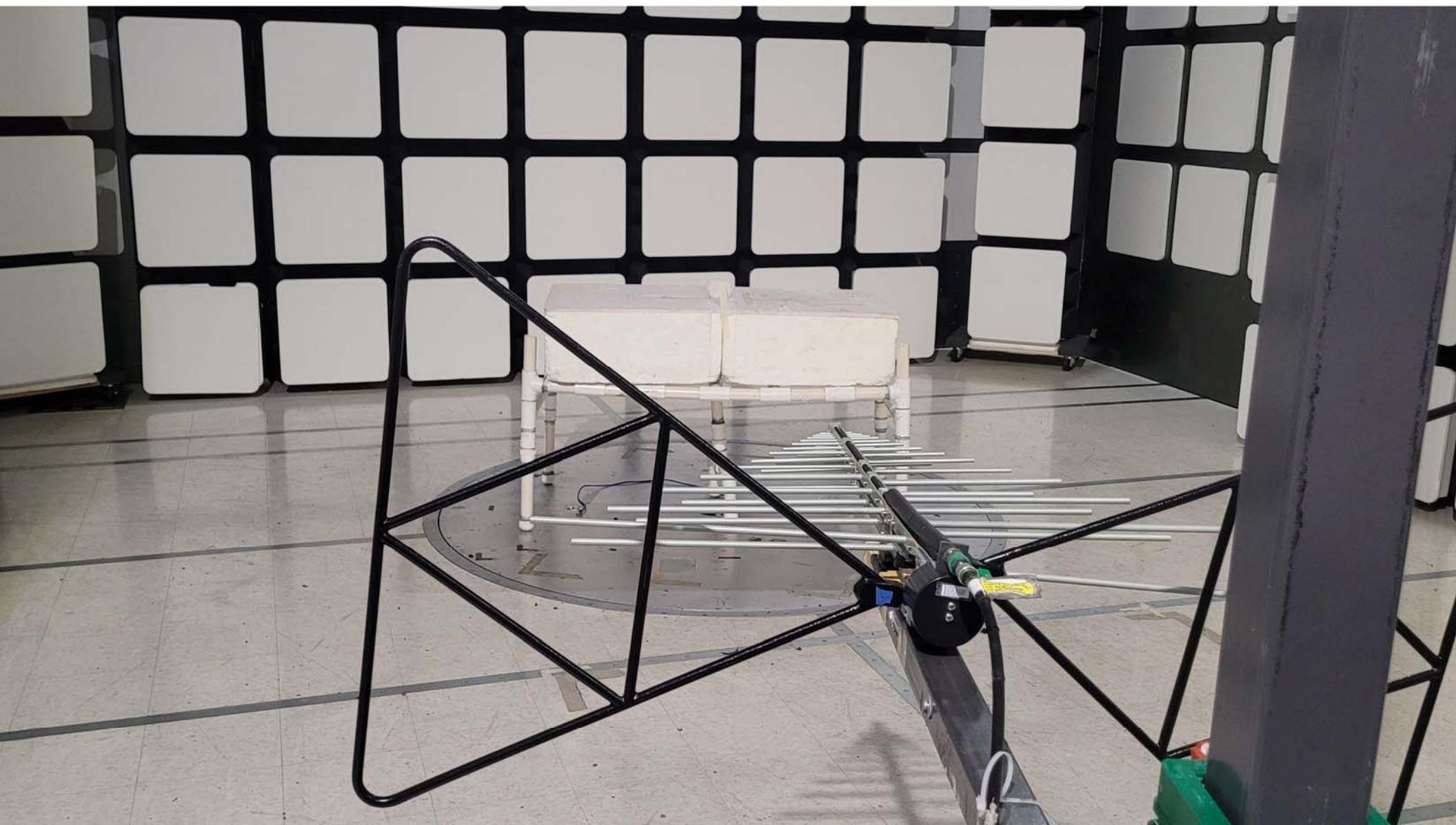
Radiated Emissions - Below 1 GHz - Rear View
