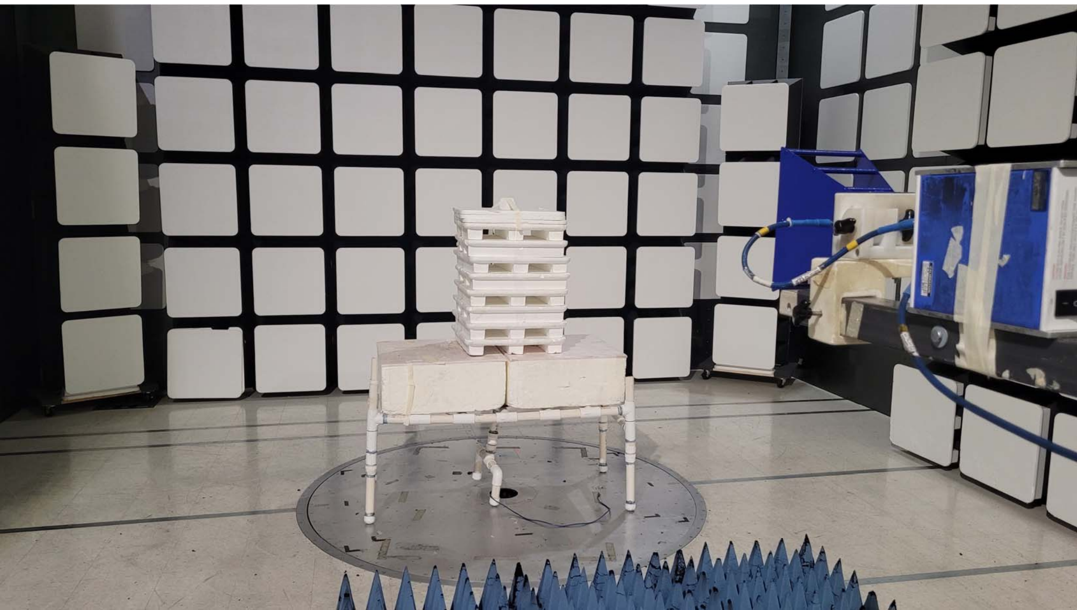
Radiated Emissions - Above 1 GHz - Rear View
