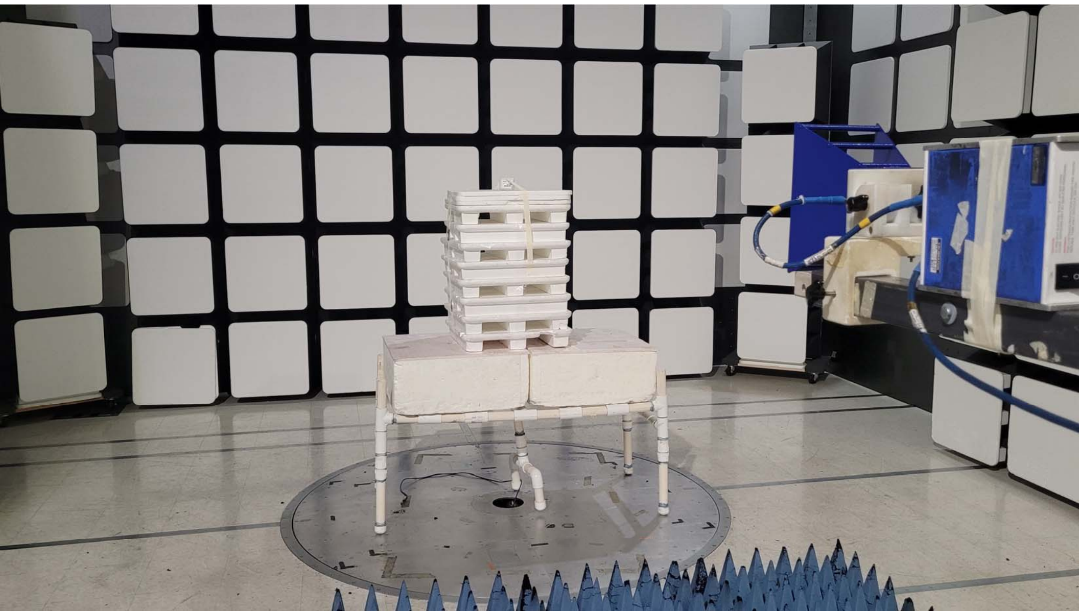
Radiated Emissions - Above 1 GHz - Front View
