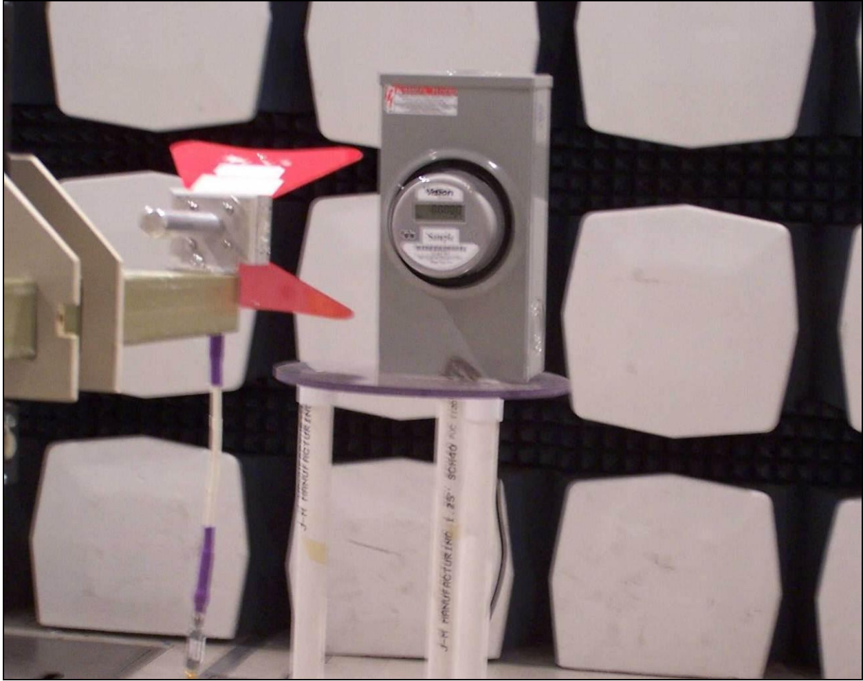
Photograph 2. Radiated Spurious Emissions Test Setup
