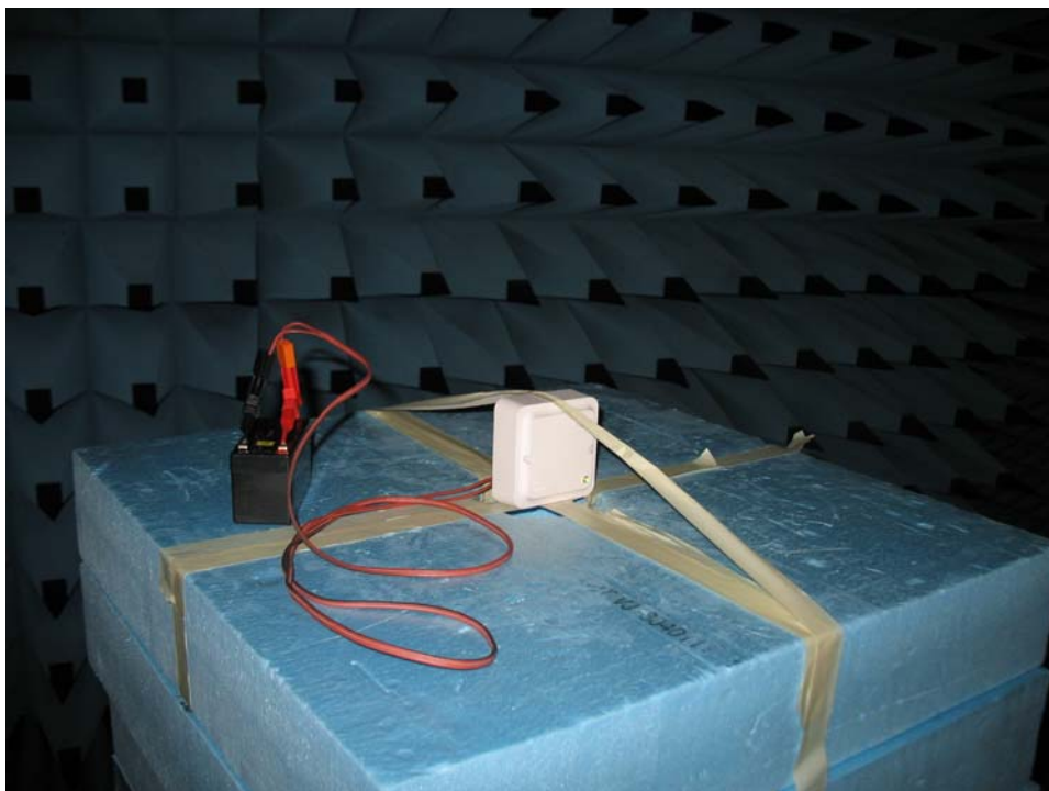
Radiated spurious emission above 1-26 GHz
