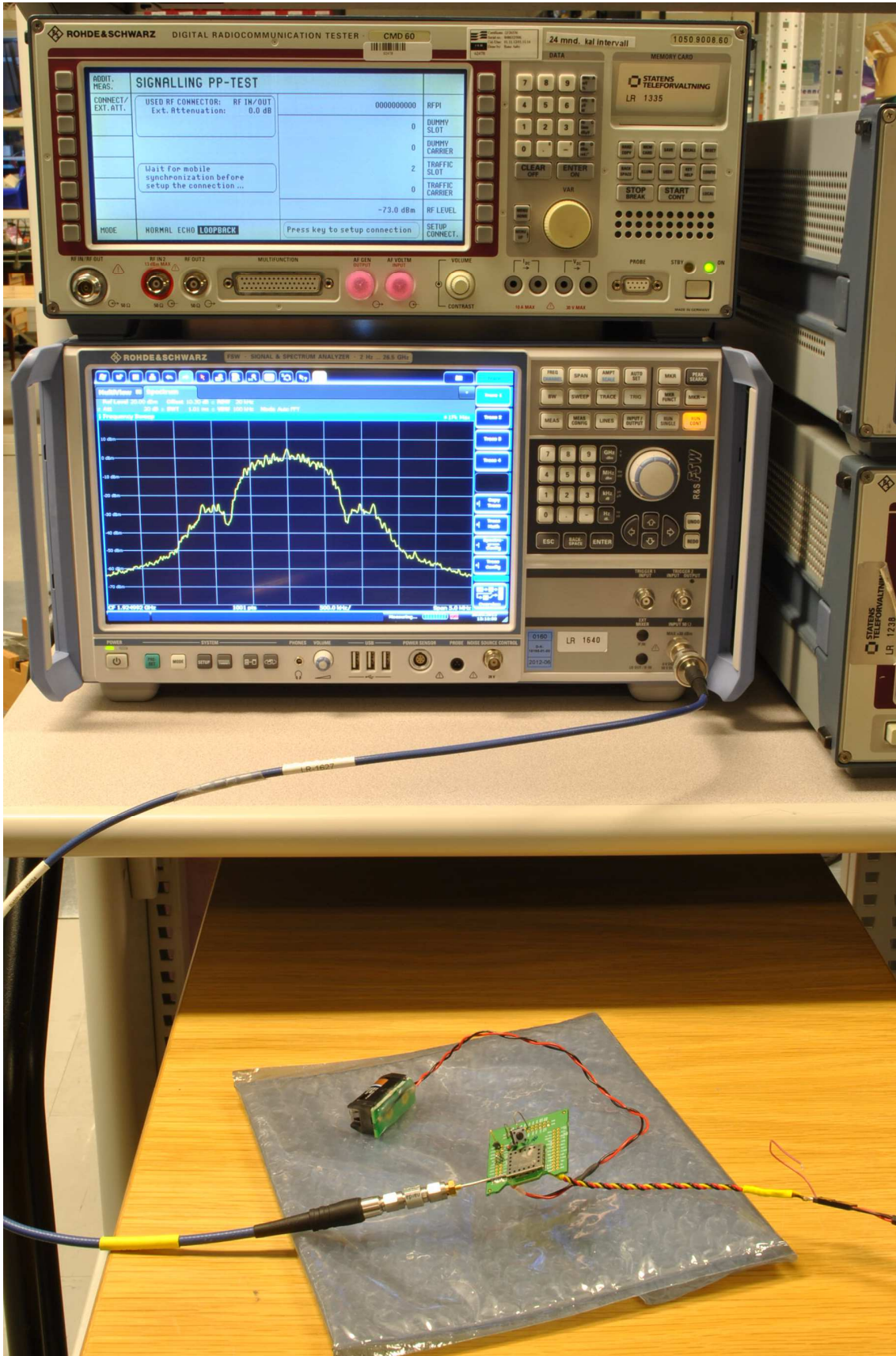
Conducted Tests
