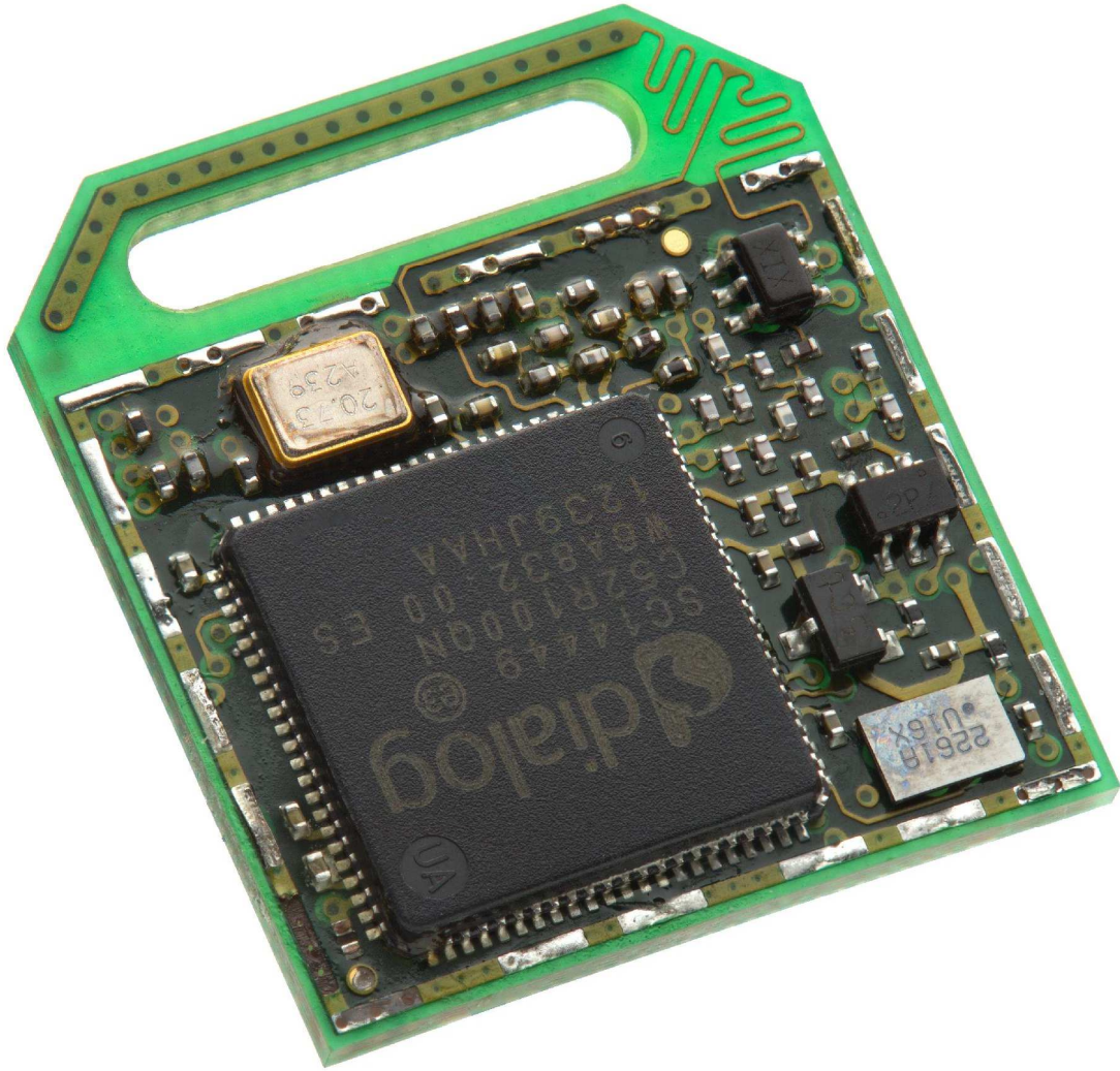
Module – Front, without shielding
