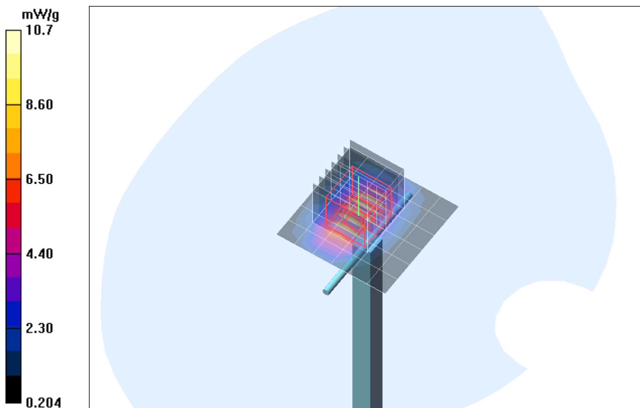
Fig. 9: Validation measurement 1900 MHz Body (March 14, 2011), coarse grid. Ambient Temperature: 21.8° C, Liquid Temperature: 21.4° C.
