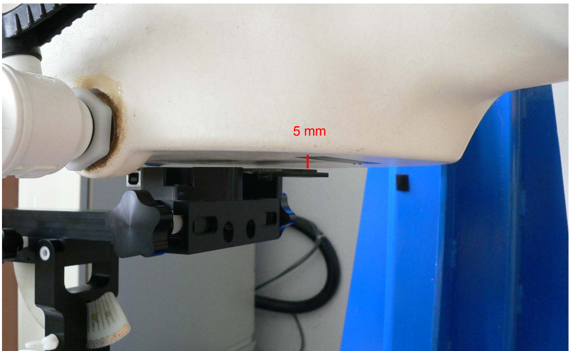
Fig. 14: Antenna 1 and 2, Position 1, 5 mm.
