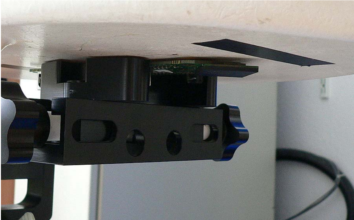
Fig. 13: Antenna 1 and 2, Position 1, 0 mm.
