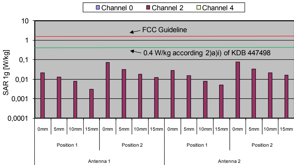
Fig. 8: The measured SAR values for the SiTel Semiconductors BV SC14CVMDECT for the US DECT standard in comparison to the FCC exposure limit.
