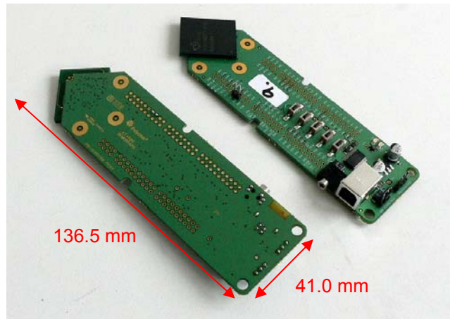
Fig. 1: Picture of the device under test.
