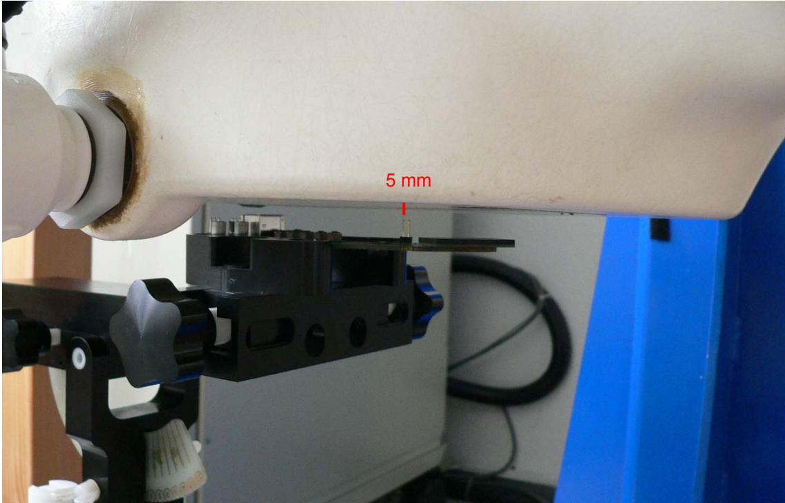
Fig. 18: Antenna 1 and 2, Position 2, 5 mm.
