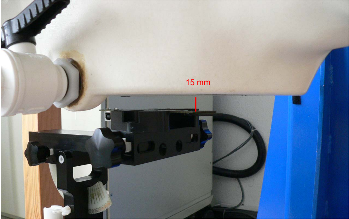
Fig. 16: Antenna 1 and 2, Position 1, 15 mm.
