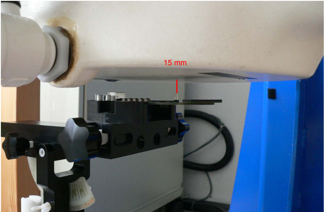
Fig. 20: Antenna 1 and 2, Position 2, 15 mm.
