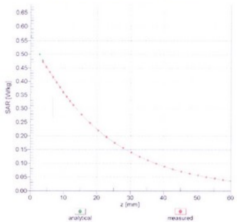
f = 750 MHz, WGLS R9 (H_convF)
