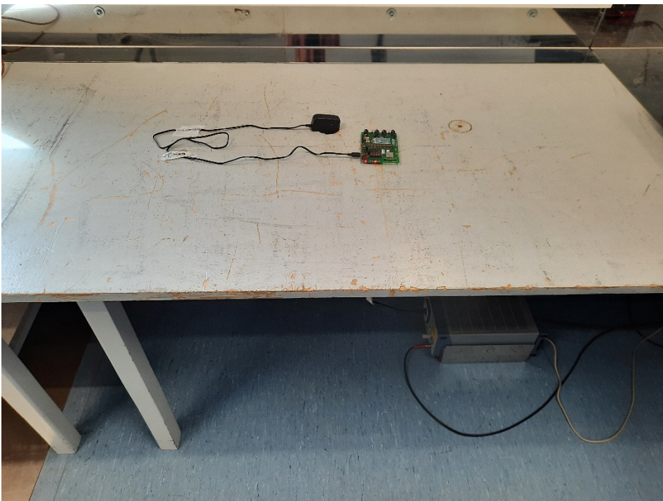
Photo 4: Conducted Emission
