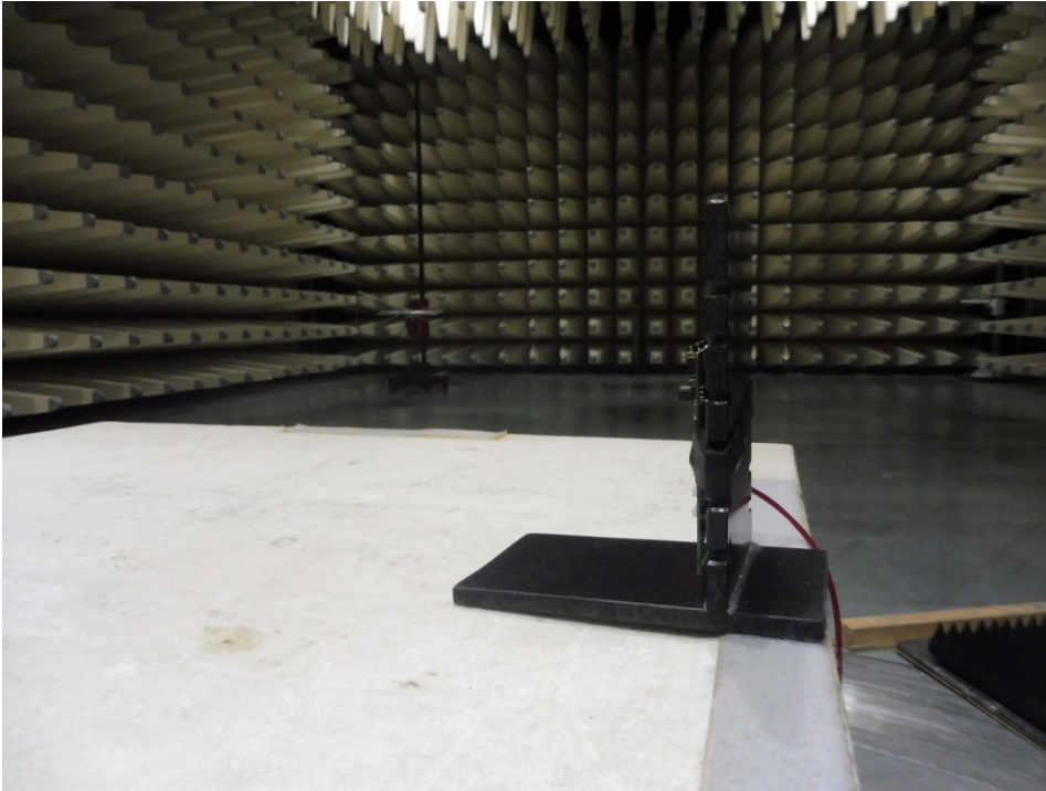
Photo 1: Radiated Emission
