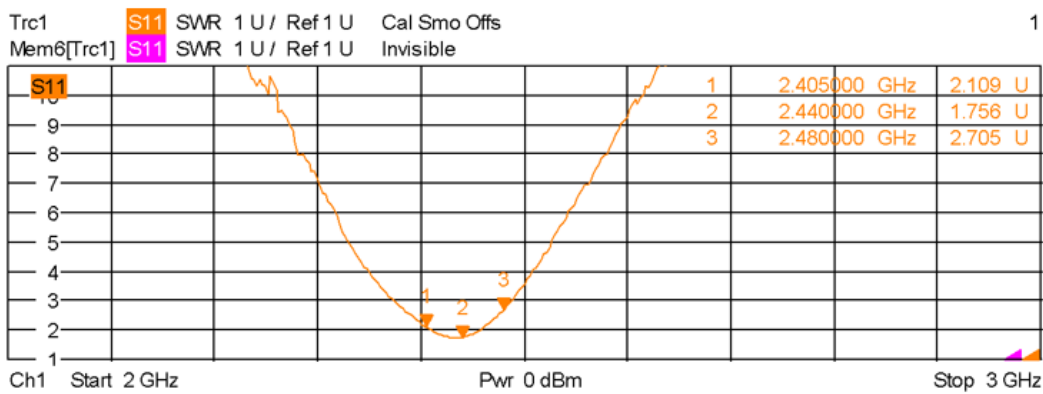
Figure 14: VSWR with Module Installed in Center (Position #2) of the Evaluation Board
