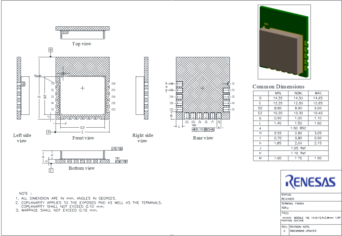
Figure 3: Mechanical Drawing
