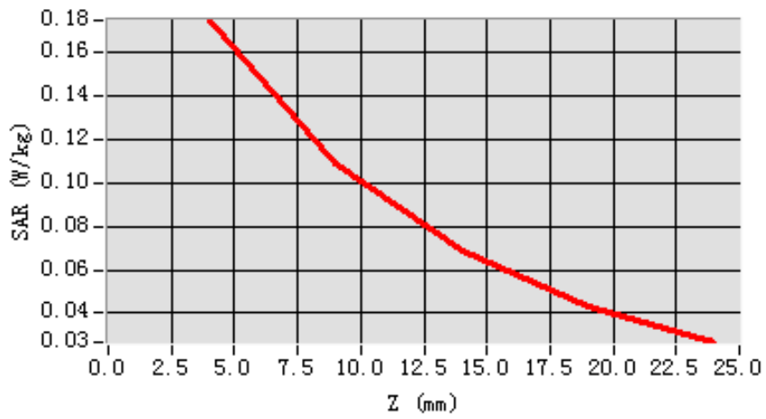
SAR, Z Axis Scan (X = -13, Y = 28)
