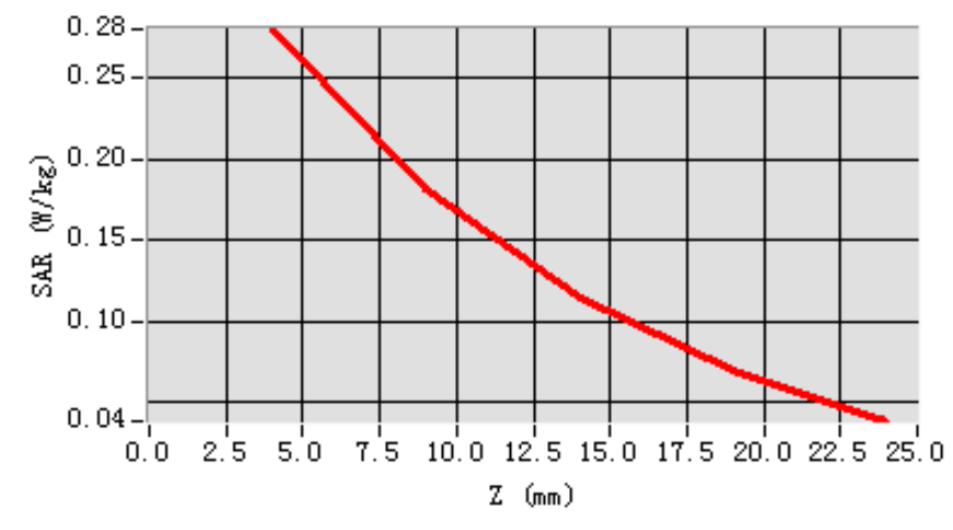
SAR, Z Axis Scan (X = -9, Y = 8)
