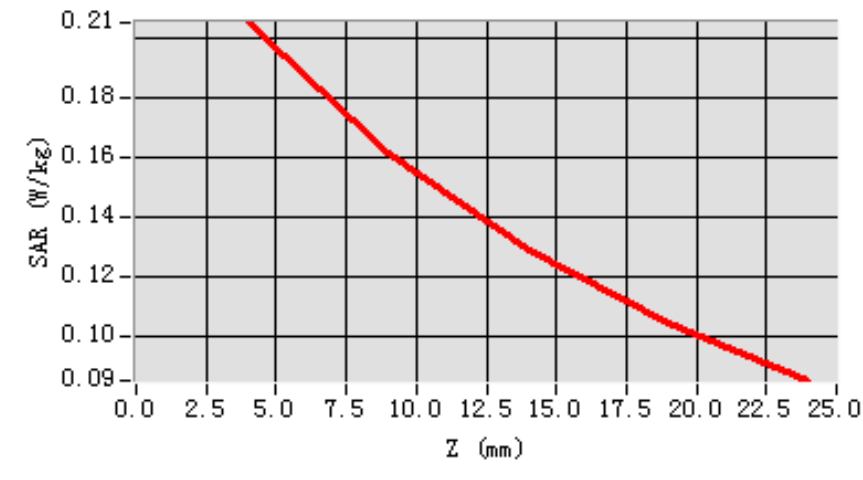
SAR, Z Axis Scan (X = -23, Y = 1)
