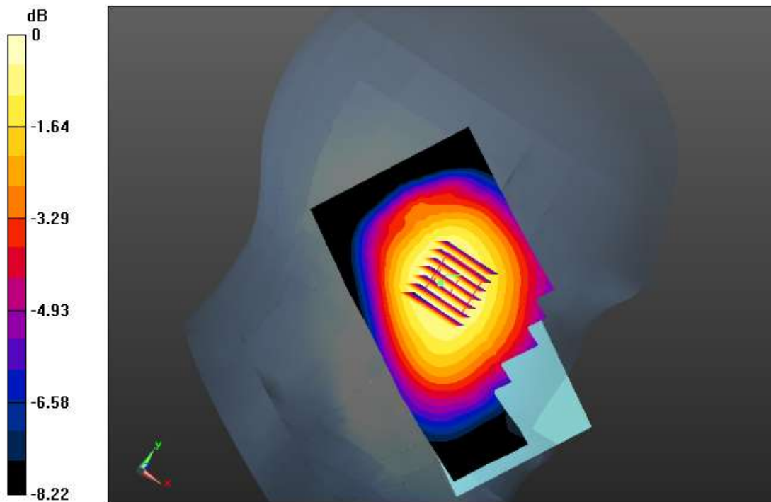
0 dB = 0.142 W/kg = -8.48 dBW/kg
