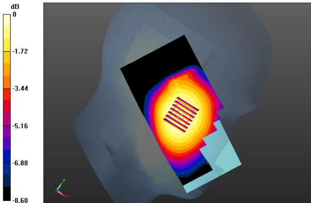
0 dB = 0.126 W/kg = -9.00 dBW/kg
