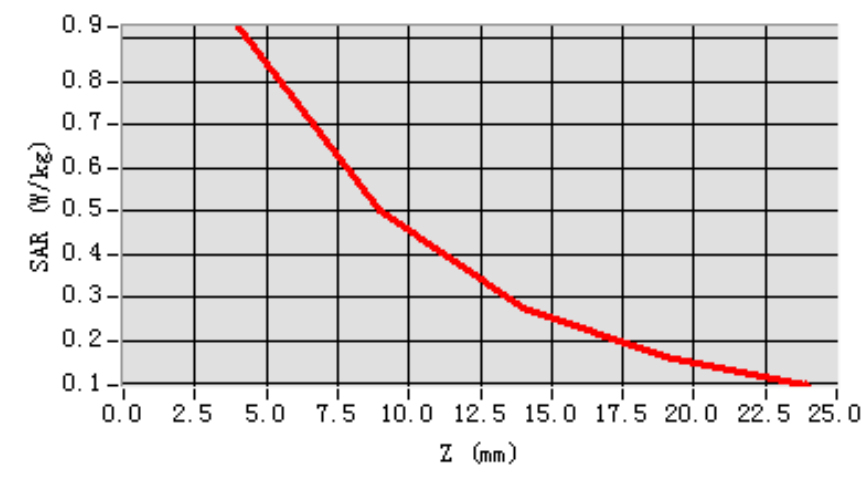
SAR, Z Axis Scan (X = 1, Y = 24)
