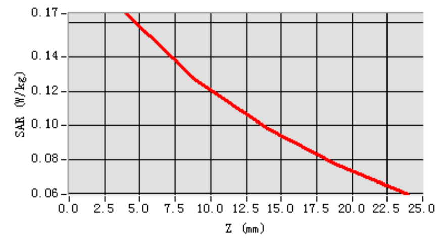
SAR, Z Axis Scan (X = 1, Y = -39)
