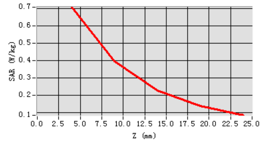
SAR, Z Axis Scan (X = 16, Y = 5)
