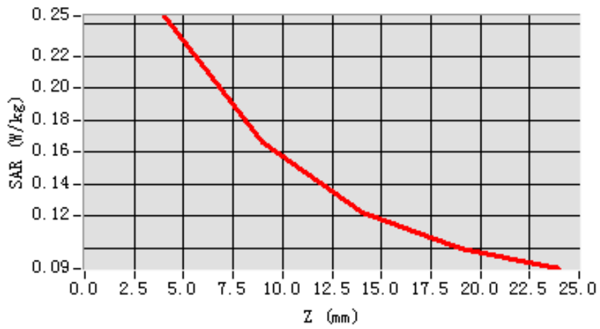
SAR, Z Axis Scan (X = -40, Y = -9)
