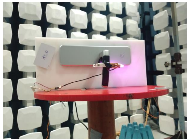
Radiated Emissions XY plane (BLE and Zigbee)
