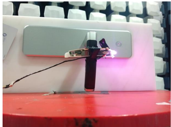
Radiated Emissions XZ plane (BLE and Zigbee)
