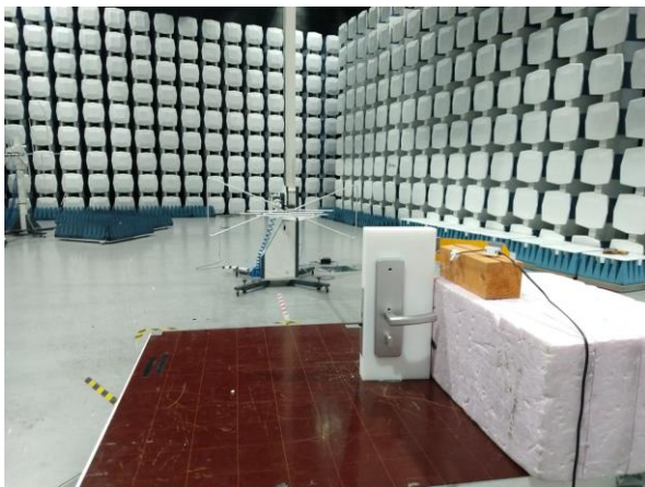
Radiated Emissions < 1 GHz (RFID)
