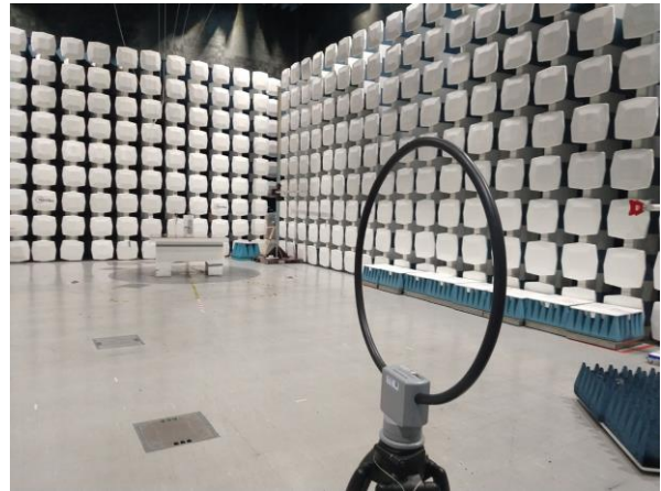
Radiated Emissions < 30 MHz, Transverse mode (RFID)
