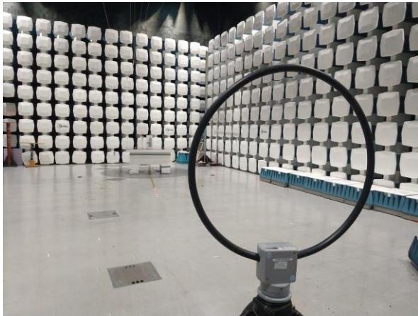
Radiated Emissions < 30 MHz, Longitudinal mode (RFID)
