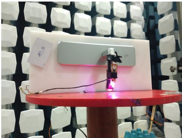
Radiated Emissions YZ plane (BLE and Zigbee)
