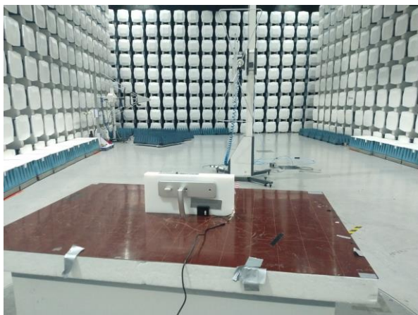
Radiated Emissions < 1GHz (BLE and Zigbee)
