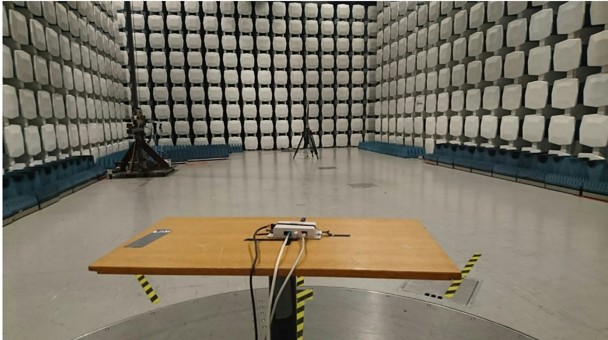
Radiated < 30MHz
