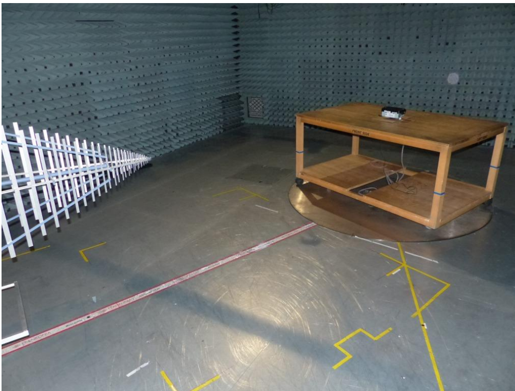
Photo 2: Test setup for radiated measurements (Enclosure, semi-anechoic chamber, 30 MHz to 1 GHz, intentional radiator §15)
