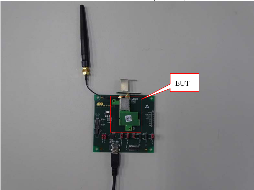
Detail of test fixture & EUT (EMIP400)
