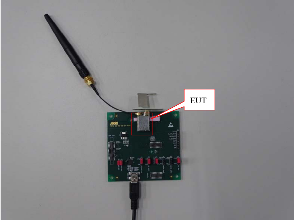
Detail of test fixture & EUT (EMIP400s)
