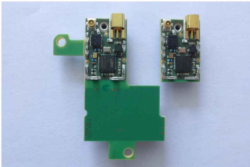
Top Layer of EMIP400(left) and EMIP400s (right)
