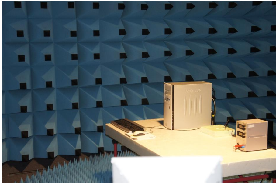
Picture 2: EUT test setup radiated emission test >1GHz (front view)
