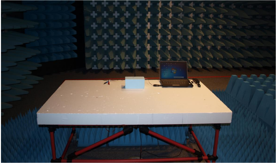
Picture 1: Test setup radiated emission (front view)
