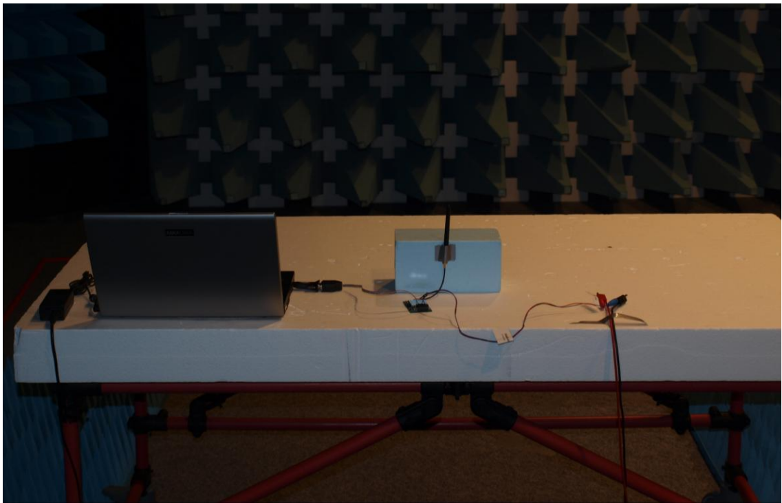
Picture 2: Test setup radiated emission (rear view)
