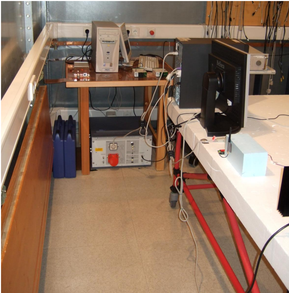
Picture 4: Test setup conducted emission (rear view)
