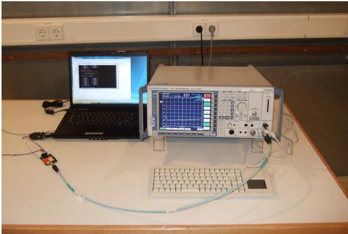
Picture 5: Test setup conducted measurement
