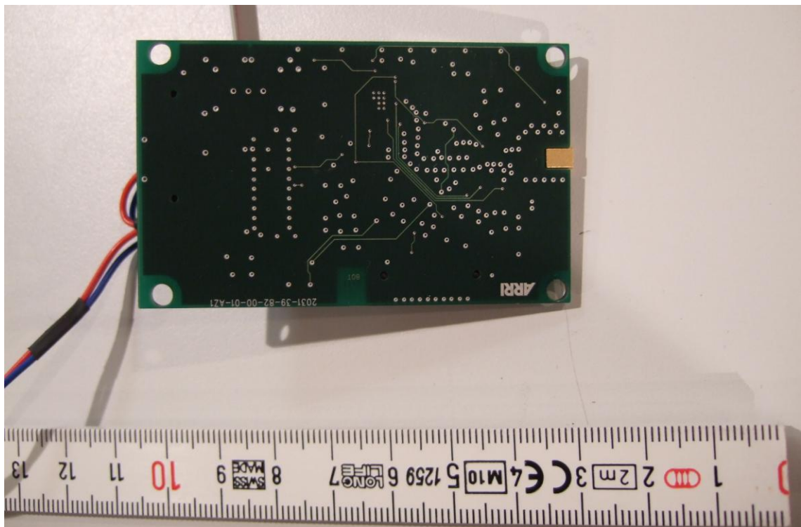
Picture 2: EUT back side
