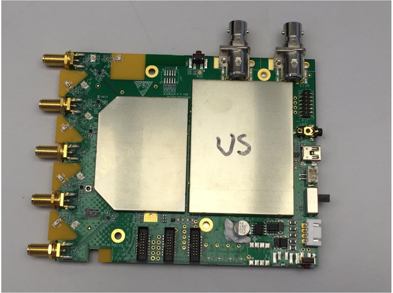
Picture 1: AMN36254_PB_ARRI_A: EUT top side
