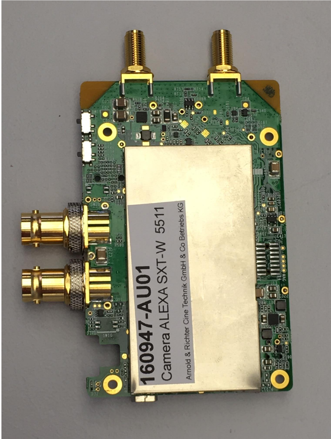
Picture 2: AMN35253_PB_ARRI_A: EUT bottom
