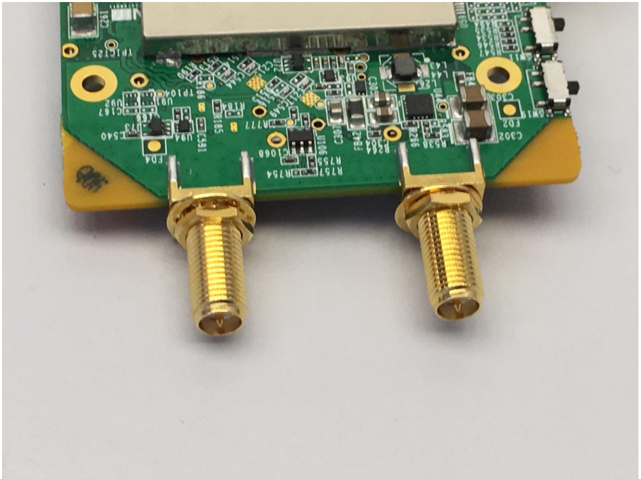
Picture 4: AMN35253_PB_ARRI_A: EUT SMA connector
