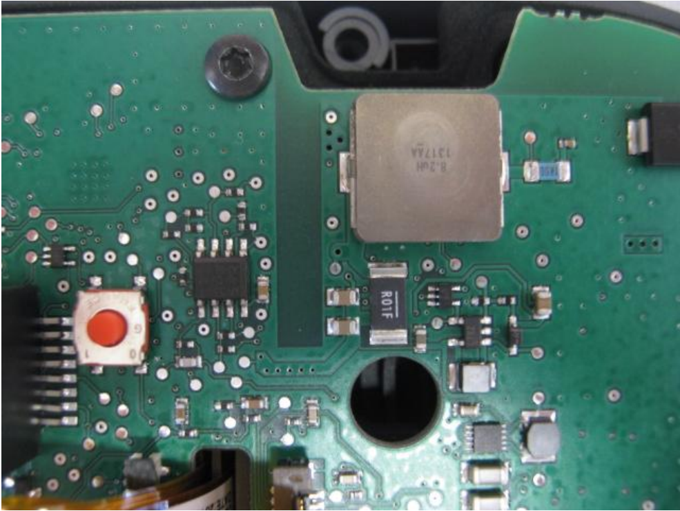
Remote radio part
