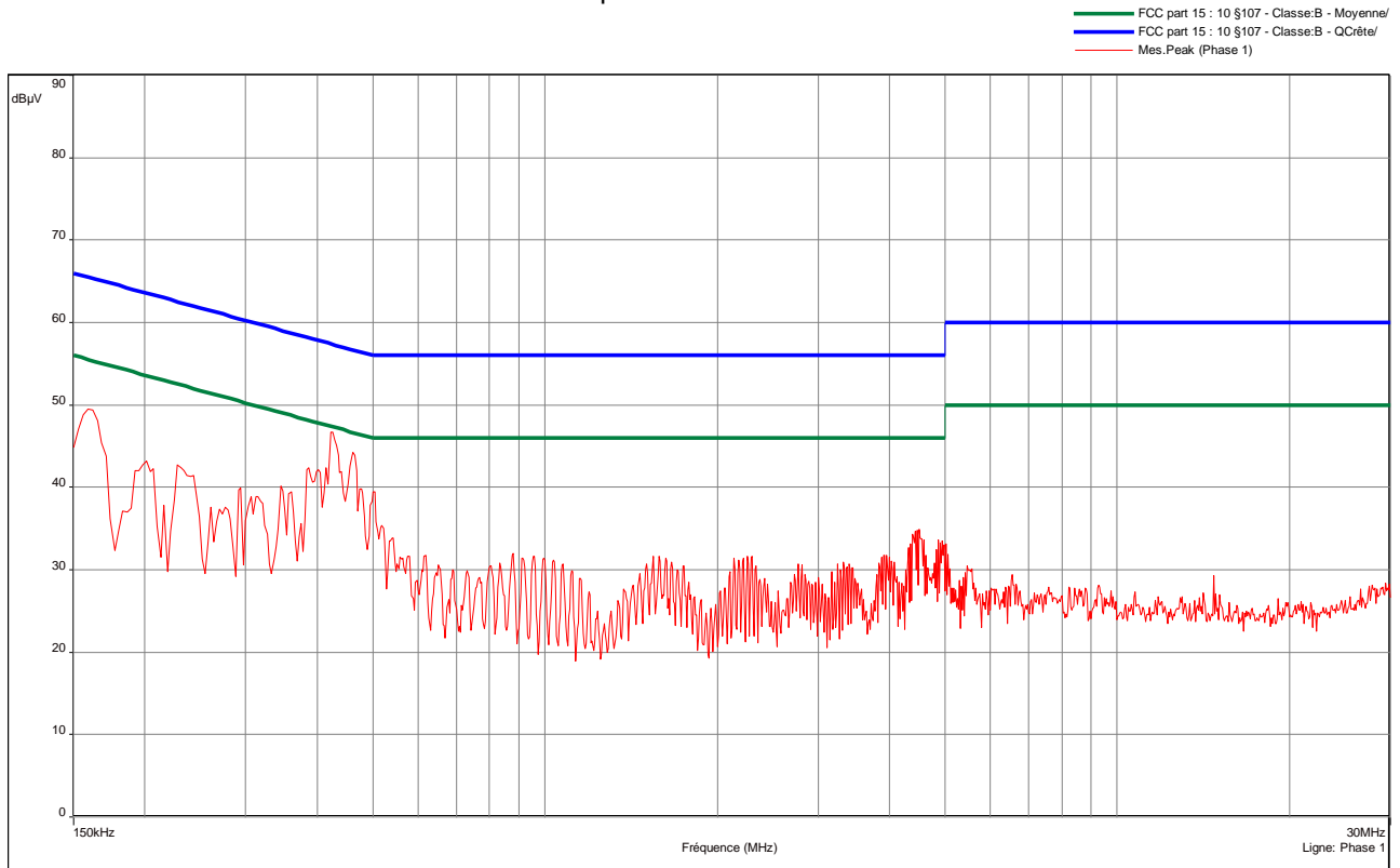
Curve N° 6: measurement on the Line with peak detector
