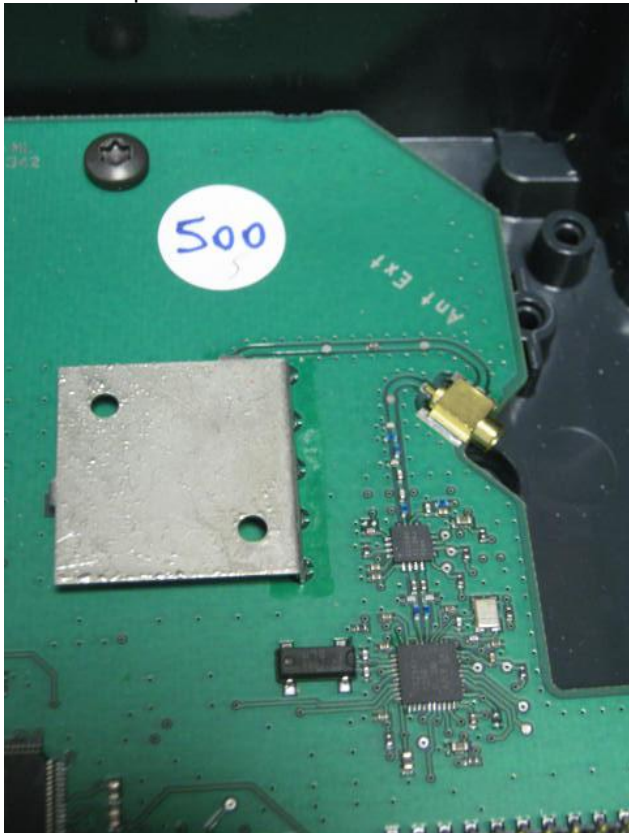
Base radio part
