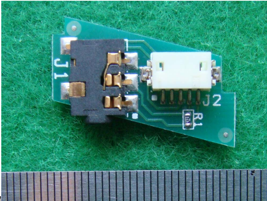
<Photograph 7: P15854 board - Front view>
