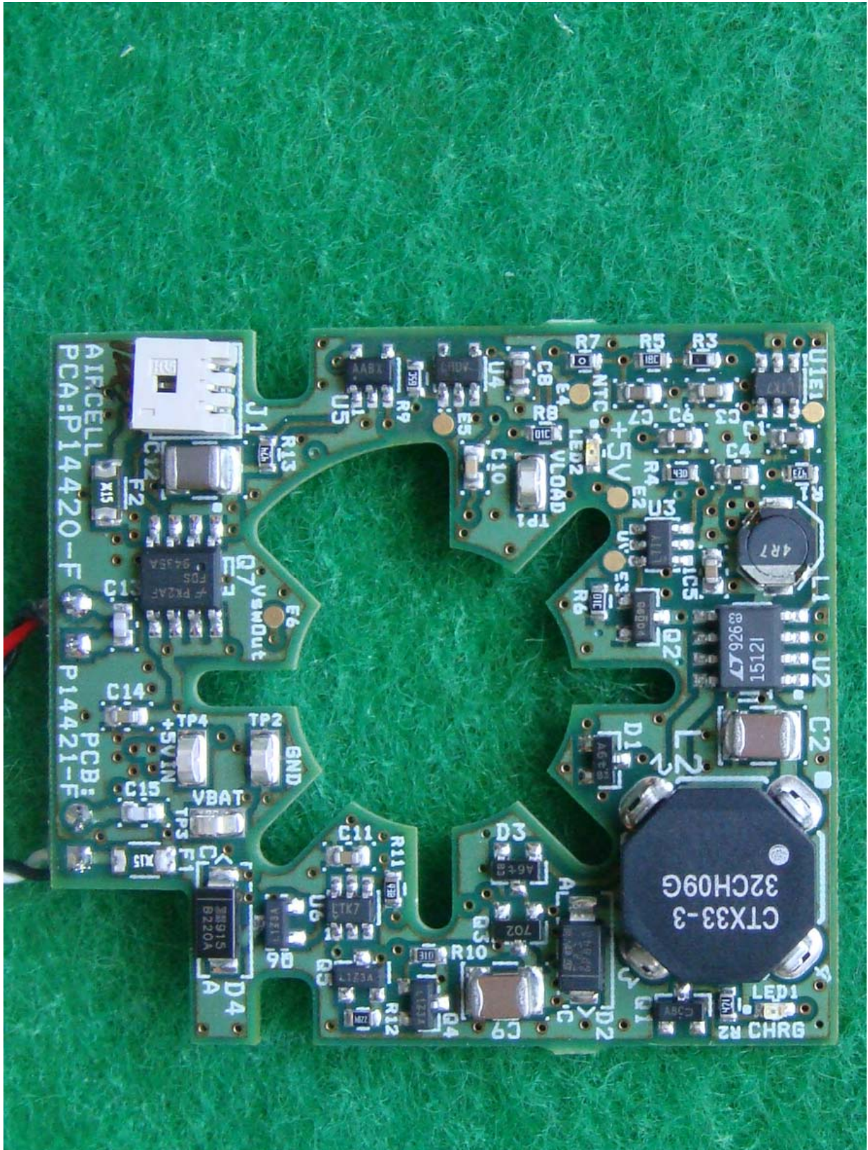
<Photograph 5: P14421-F board - Front view>
