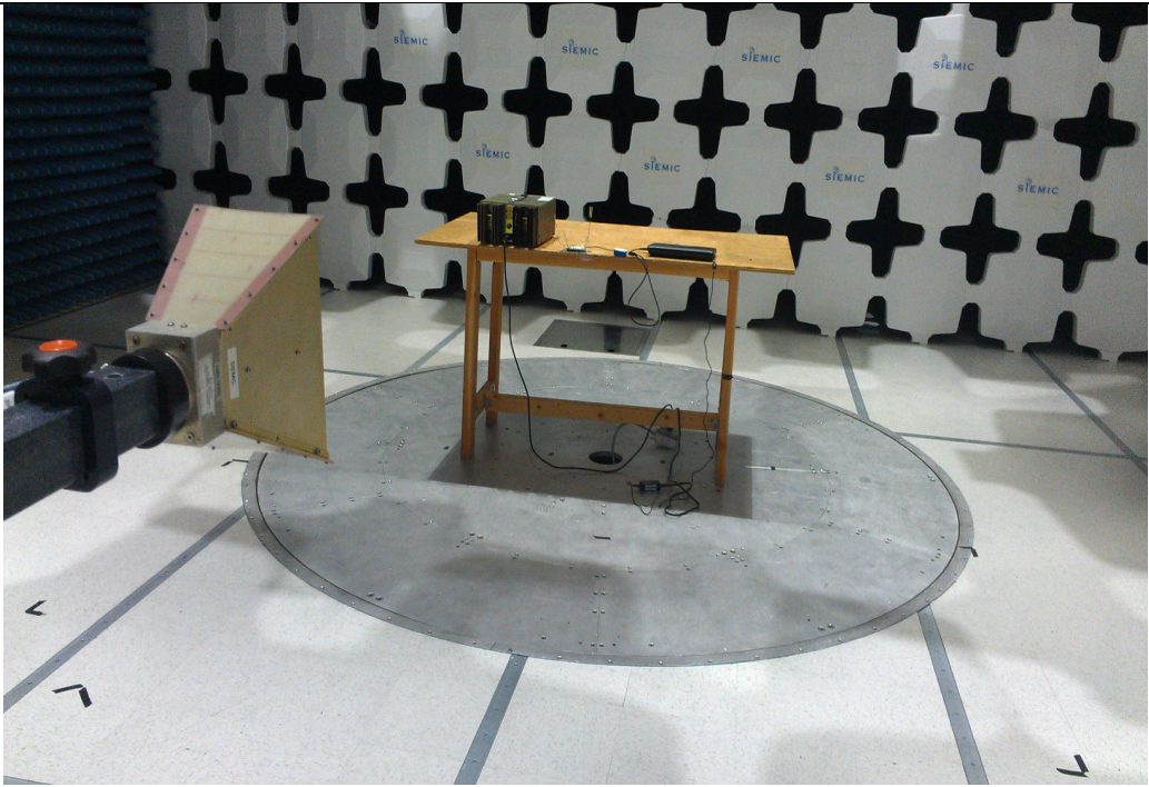
Radiated Emission Above 1 GHz Front View
