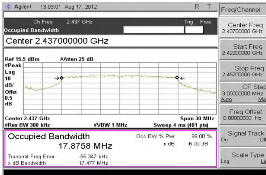
Plot - 802.11n-20MHz-2437MHz
