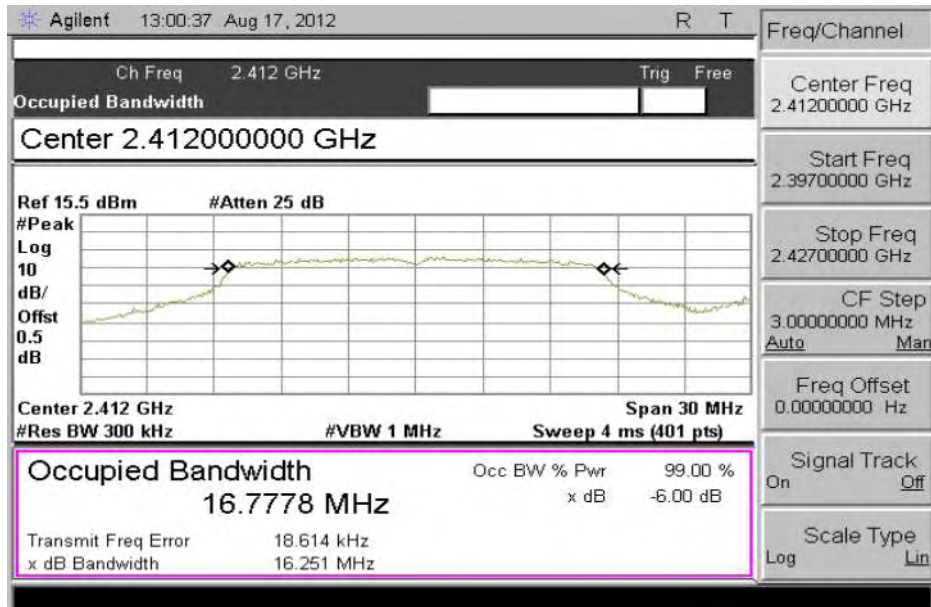
Plot - 802.11g-2412MHz
