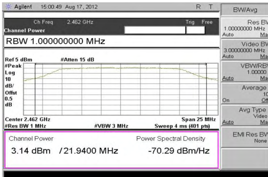
Plot - 802.11g-2462MHz
