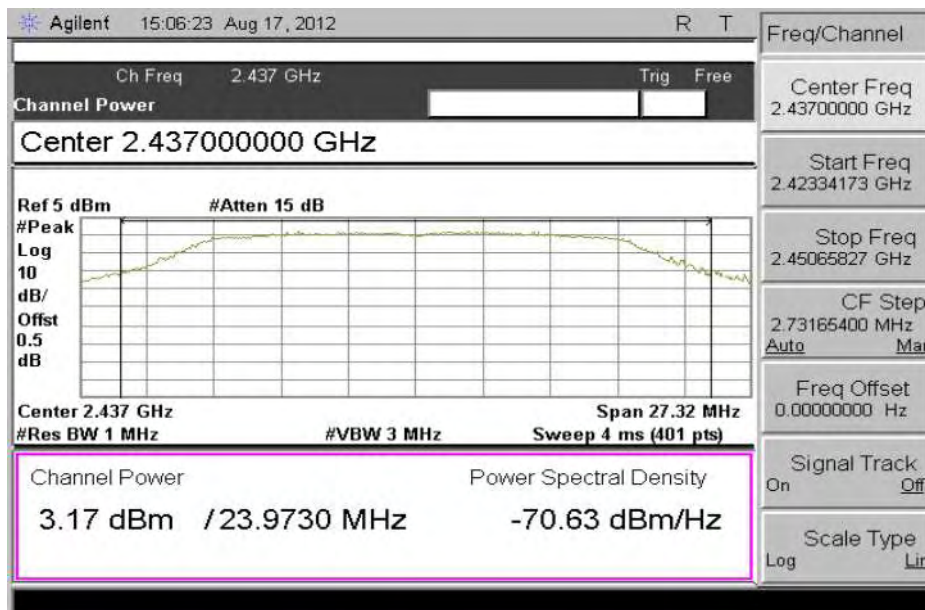
Plot - 802.11n-20MHz-2437MHz
