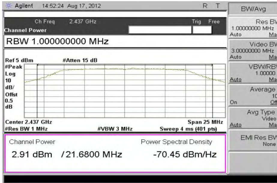
Plot - 802.11g-2437MHz
