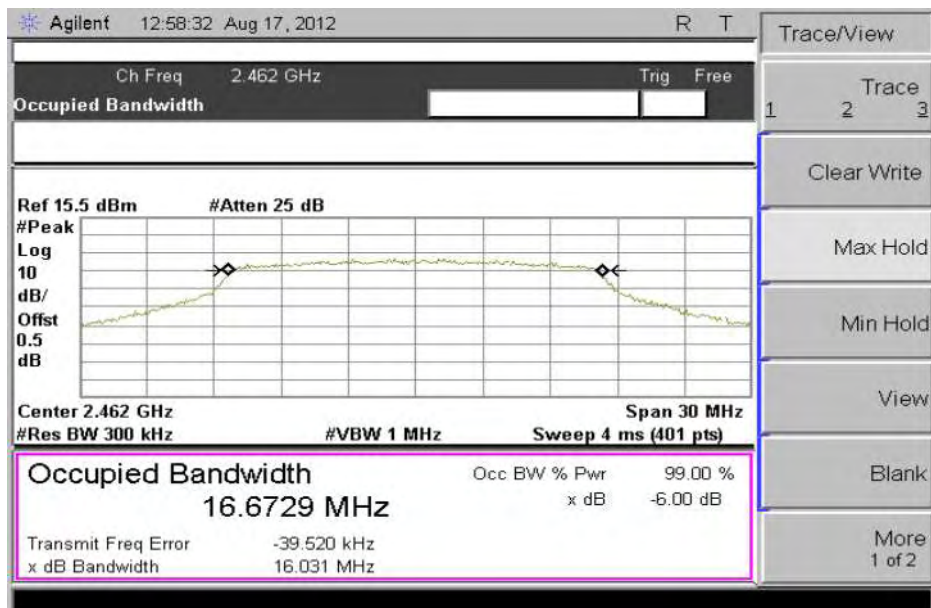
Plot - 802.11g-2462MHz
