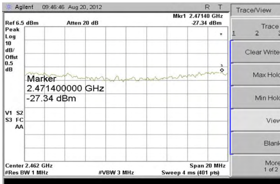
Plot - 802.11g-2462MHz
