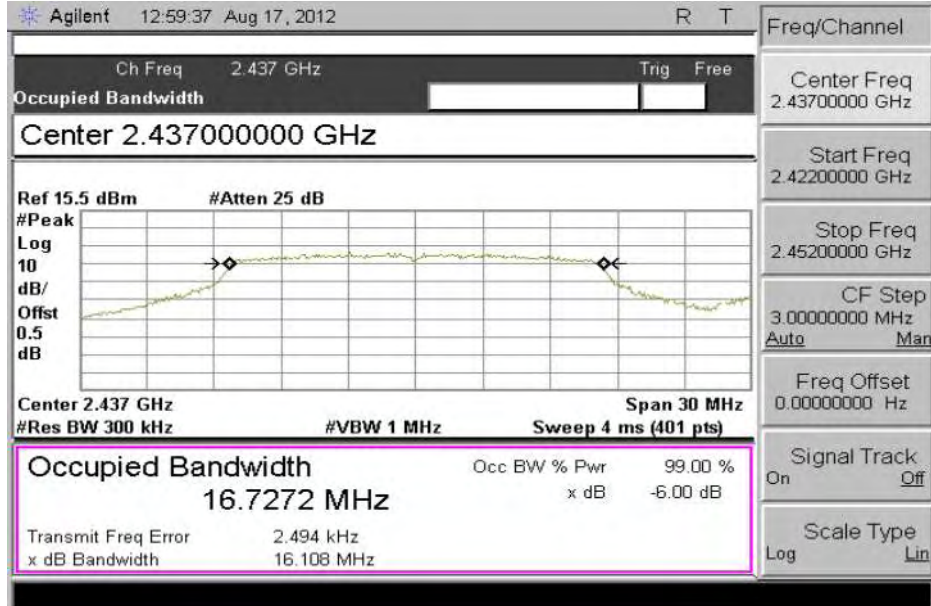
Plot - 802.11g-2437MHz
