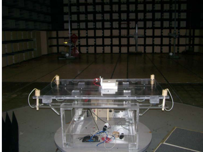
Figure 3. Set up of Radiated Emission (rear)
