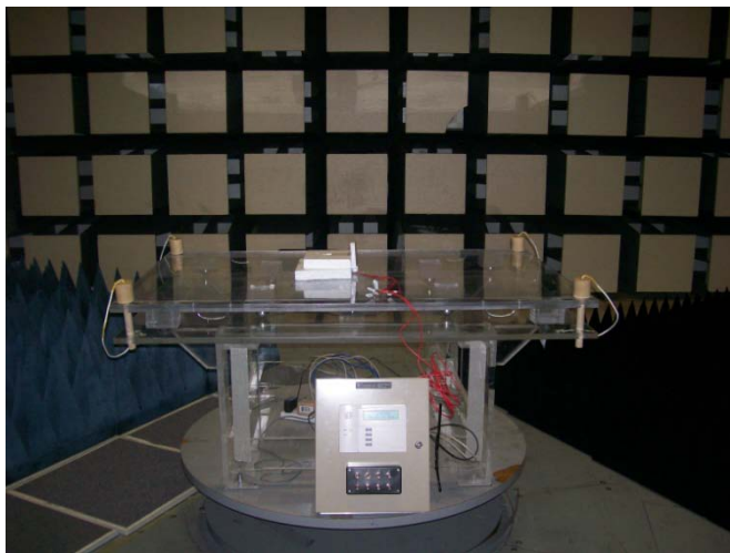
Figure 4. Set up of Radiated Emission (front)
