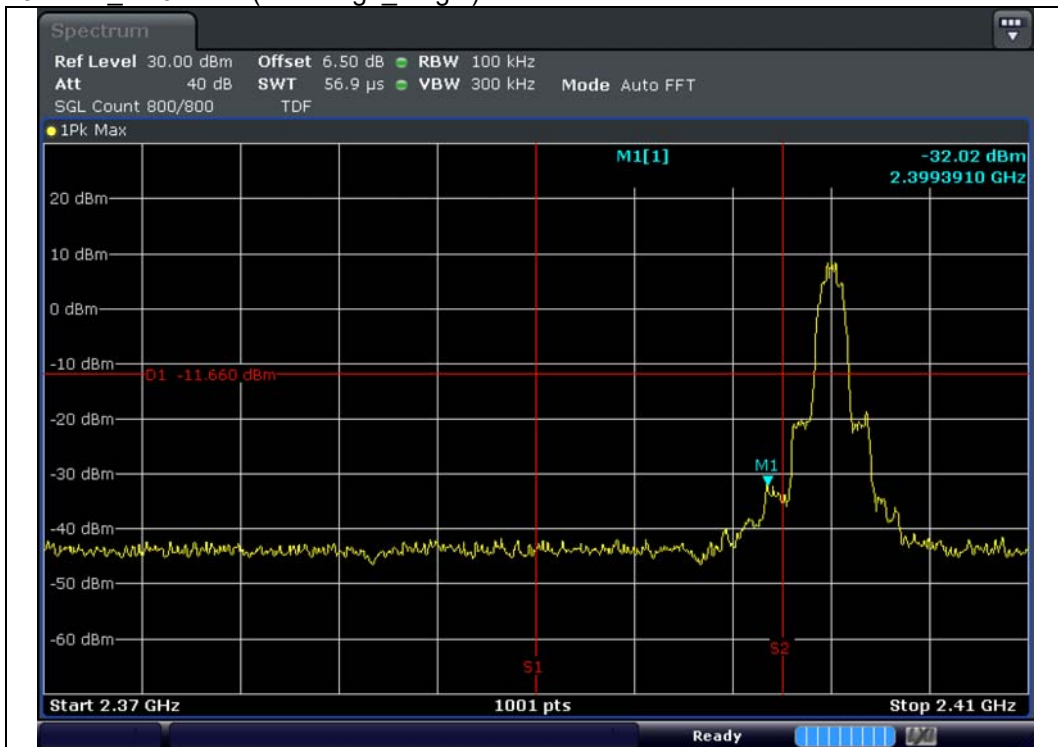
8DPSK_2_402 MHz(Bandedge_Single)
