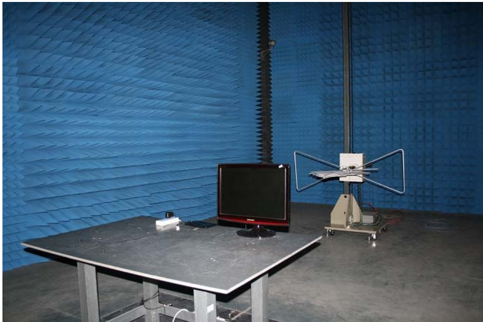
Radiated Emissions
