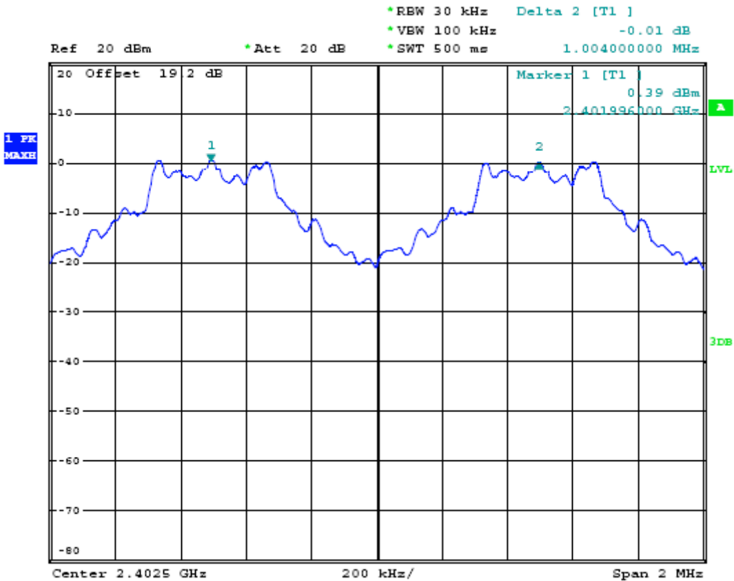
TEST PLOT FOR FREQUENCY SEPARATION –CHANNEL0-1(1Mbps)
