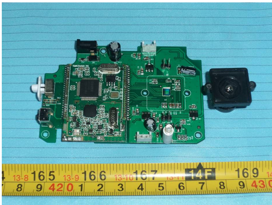
EUT – Main Board Top with Camera off View
