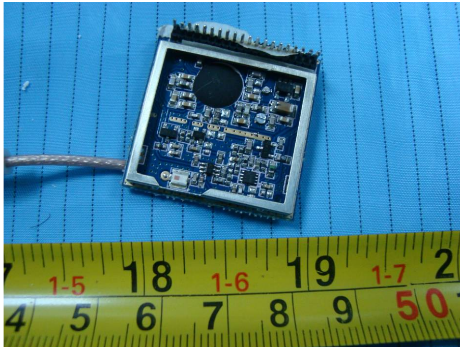
EUT – RF Board Shielding off Top View
