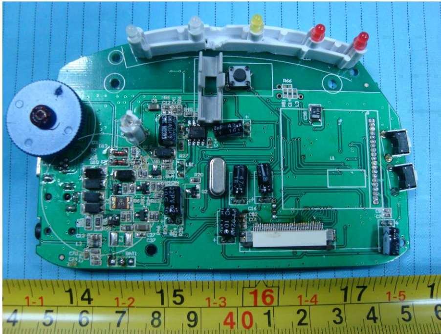
EUT – Main Board without RF Module Bottom View
