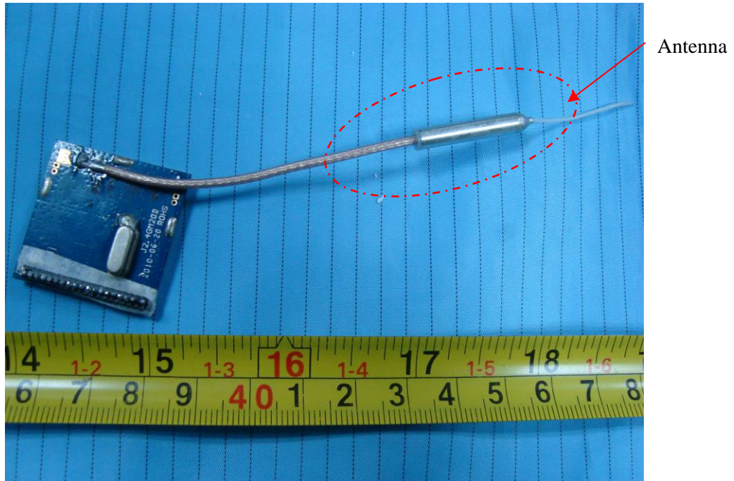
EUT – RF Board Bottom View
