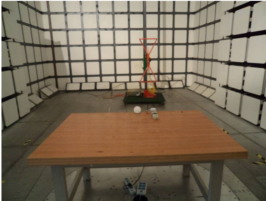
Radiated Emissions View (30MHz~1000MHz)
